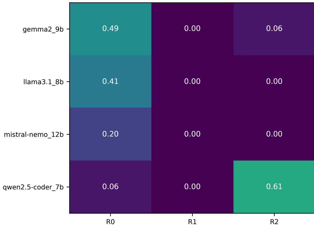
distinguishing_trace full
