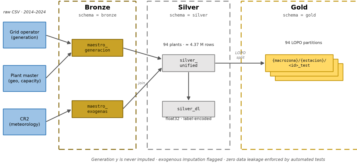
Fig. 1. Medallion ETL data-lineage. Source systems feed two Bronze master tables, joined into silver_unified and its numeric silver_dl view; the gold layer holds one LOPO test partition per plant. Generation is never imputed, and zero leakage is enforced by automated tests.
