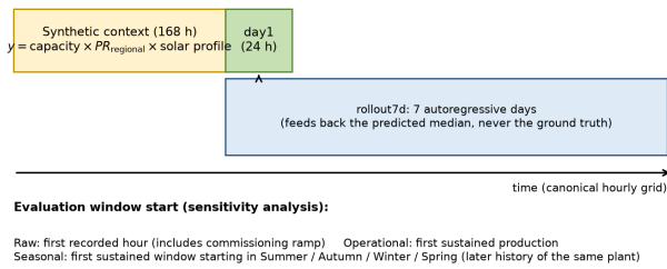
Fig. 2. Zero-shot Cold-Start evaluation protocol. A 168-hour synthetic context seeds the inference; the model then predicts the day1 (24 h) and rollout7d horizons. The window start defines the Raw/Operational/Seasonal sensitivity analysis.
