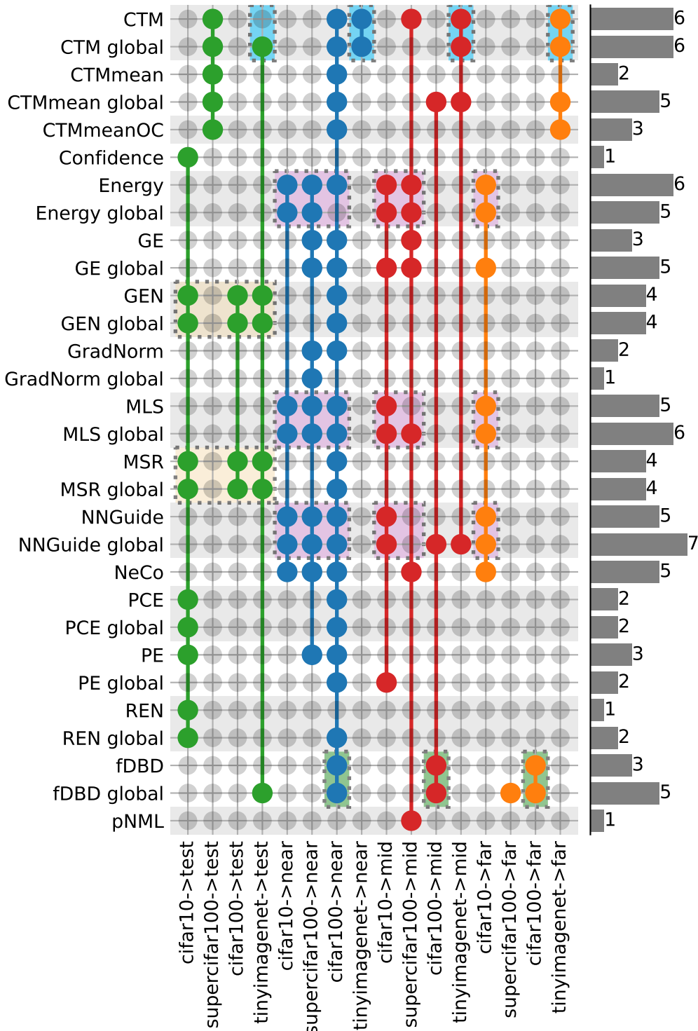
Top cliques (Backbone:Conv, Metrics=['AUGRC', 'AURC'])
