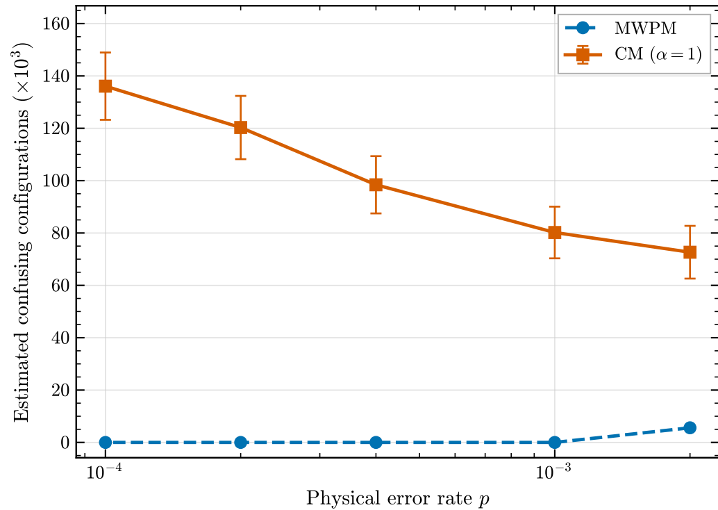
(b) d = 7 : weight-3 configurations
