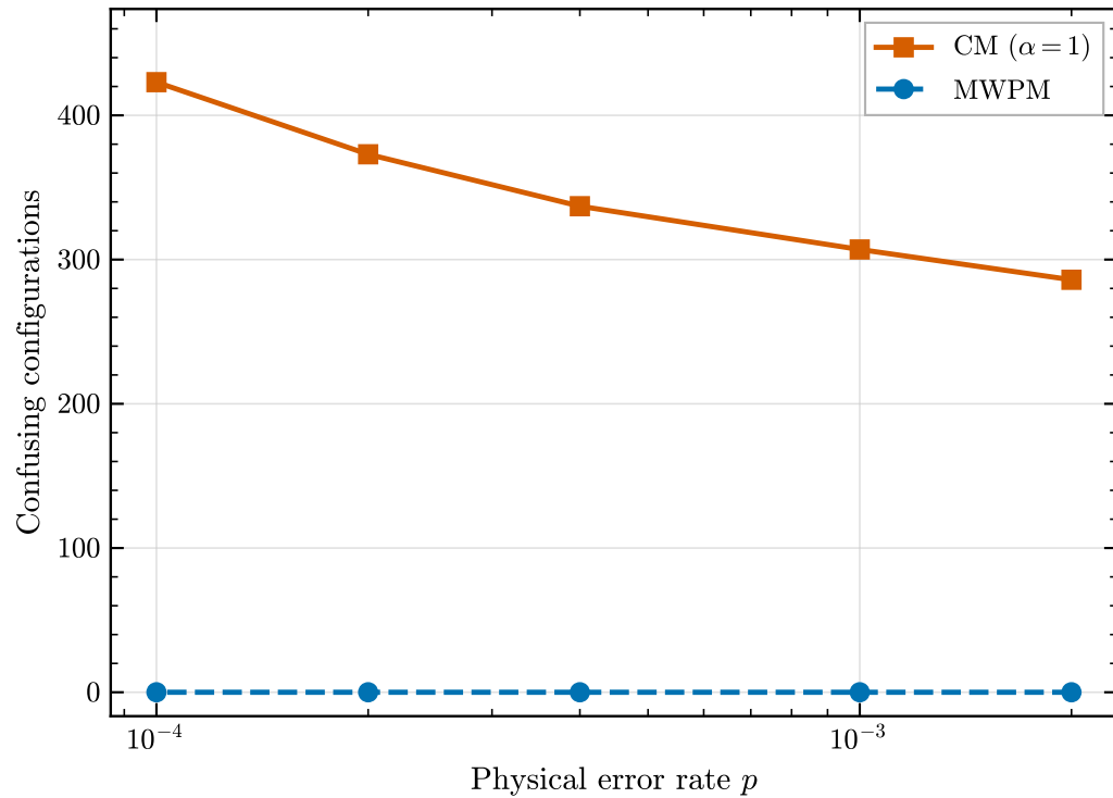
(a) d = 5 : weight-2 configurations
