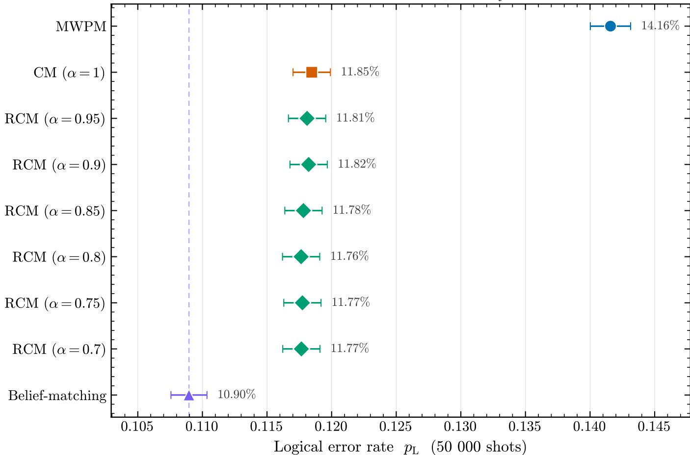
Google qec3v5 d = 5 , Z -memory, r = 5 (Spitz p_{ij} -calibrated DEM)
