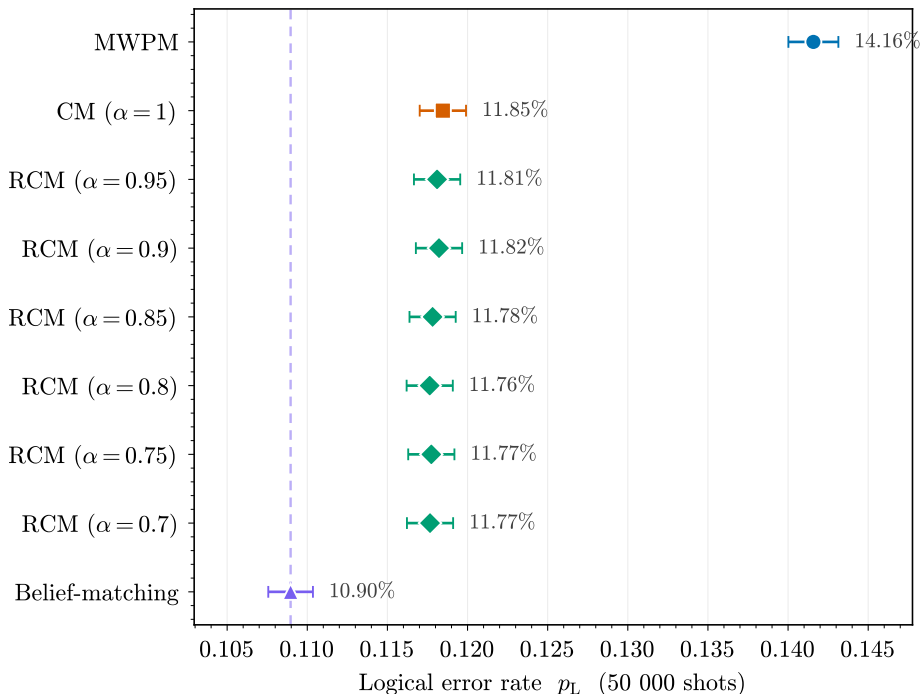
Google qec3v5 d=5 , Z -memory, r=5 (Spitz p_{ij} -calibrated DEM)
