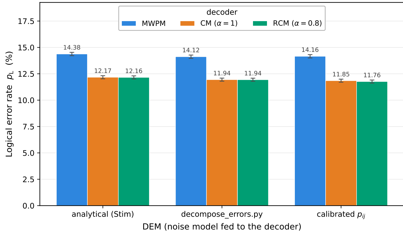
Google qec3v5 d=5, Z-memory, r=5 — 50 000 experimental shots
