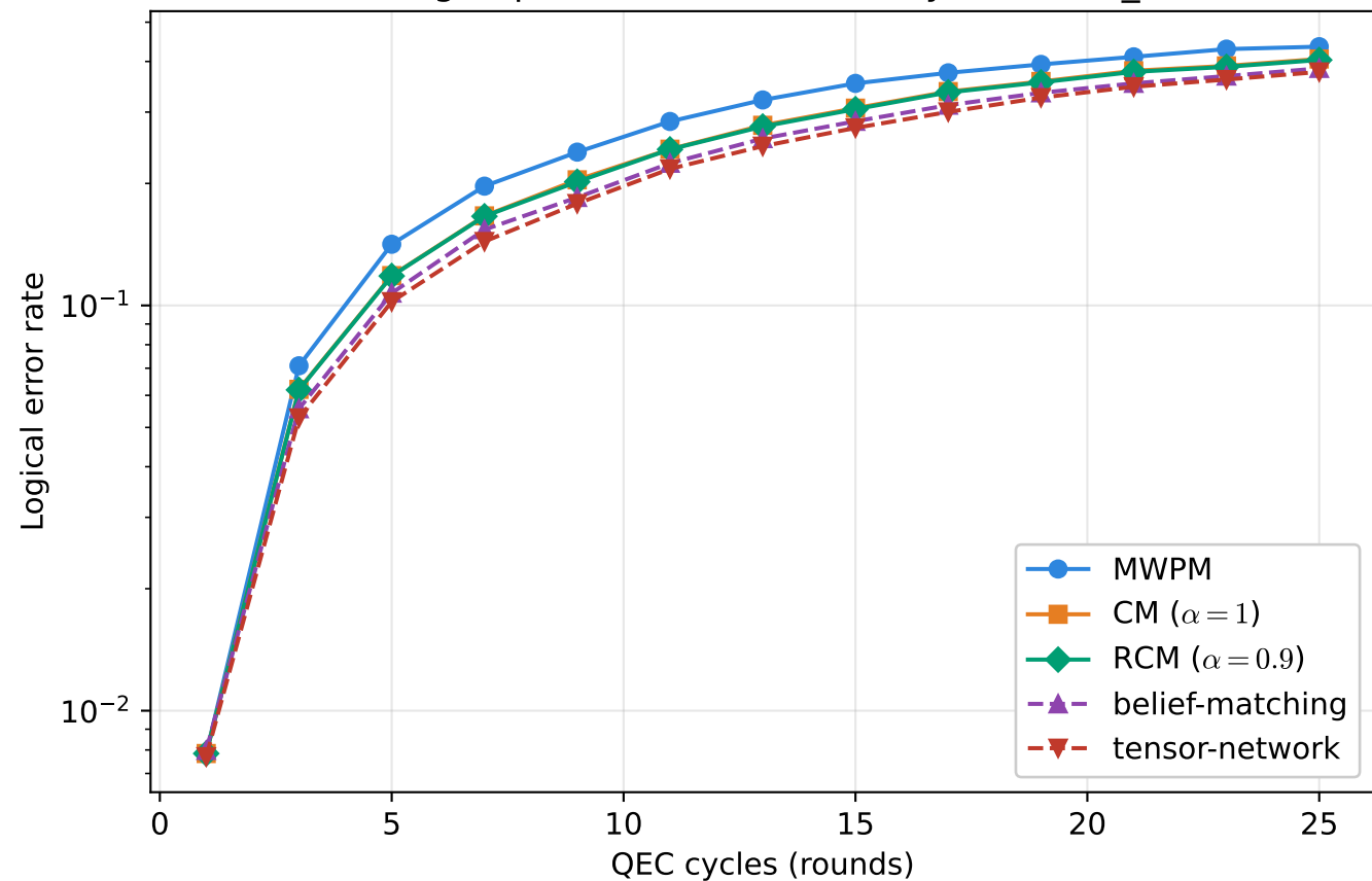
Google qec3v5, d=5 , Z-memory, center 5_5
