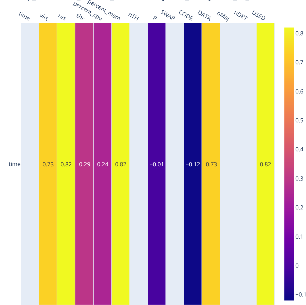
c++ - top_correlation_General_FilteredBinarytrees_binaryTrees_v6_fast
