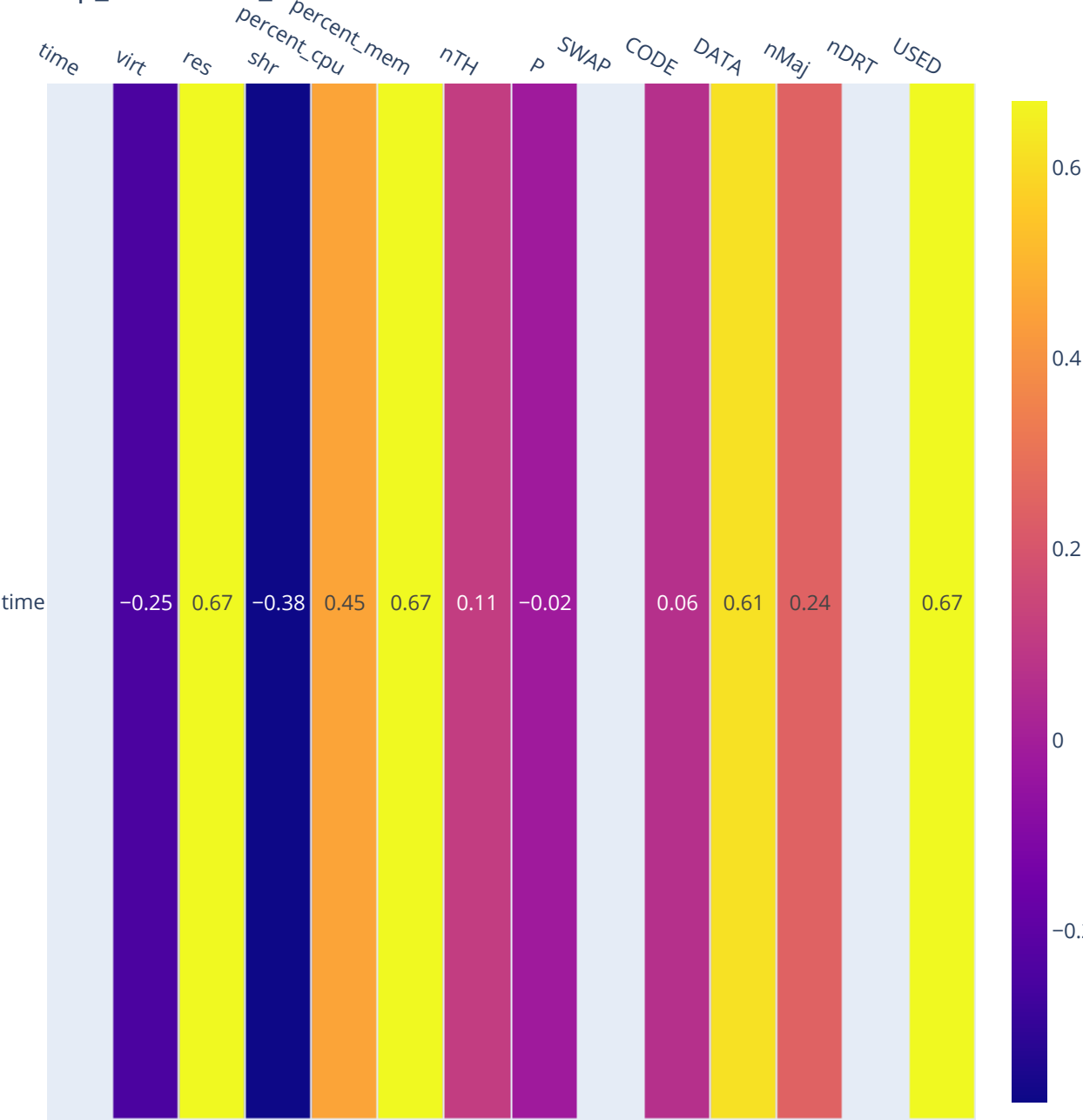
java - top_correlation_General
