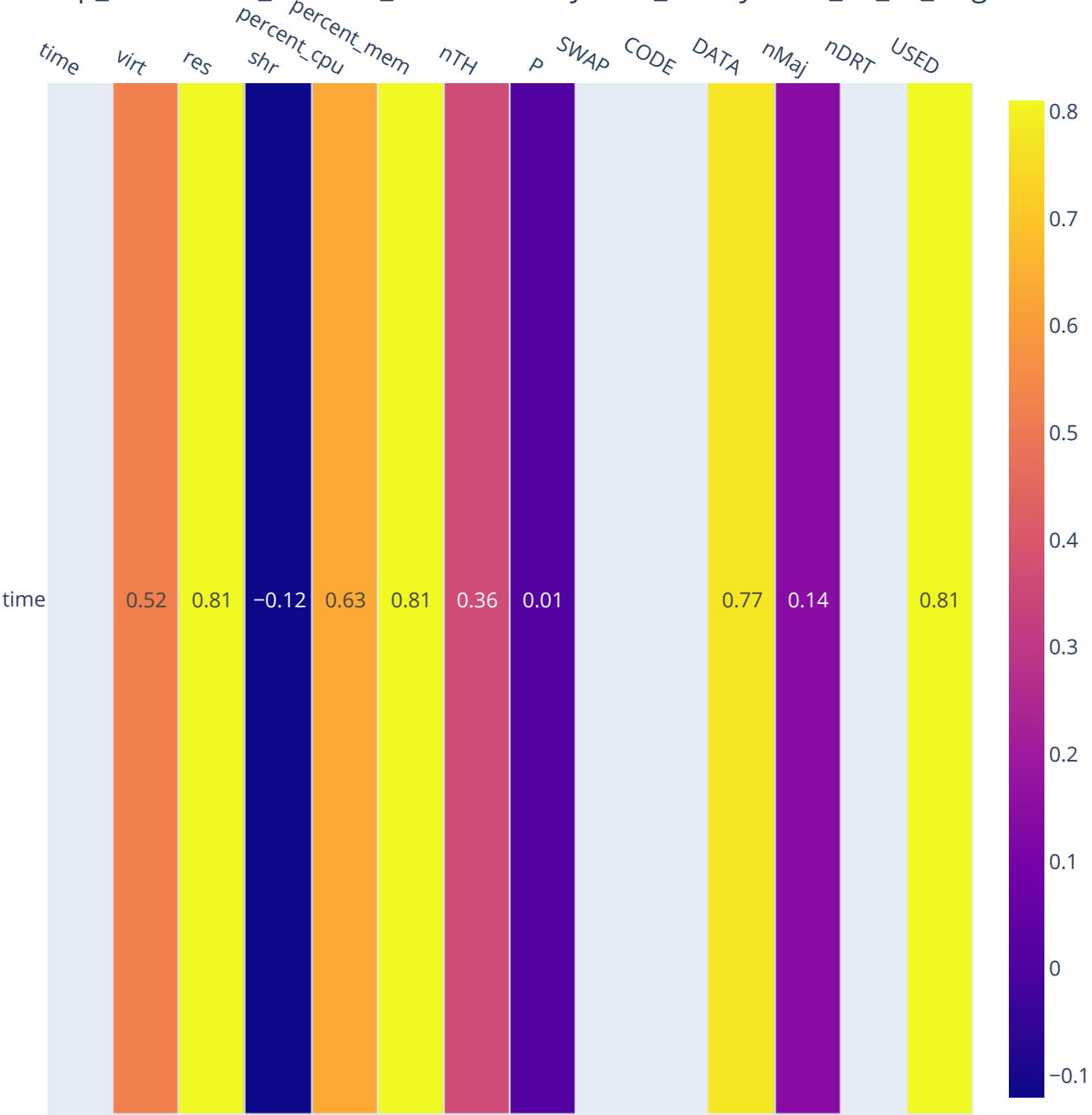
java - top_correlation_General_FilteredBinarytrees_binaryTrees_21_v4_original
