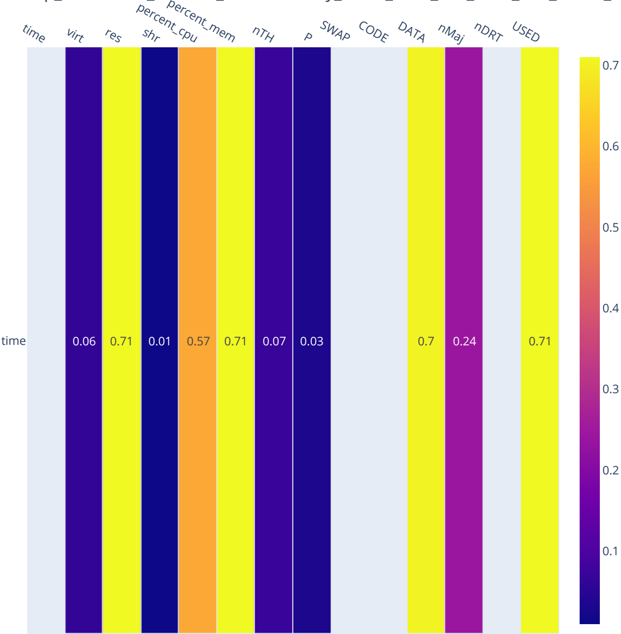
java - top_correlation_General_FilteredNbody_ONLY_1.8.0_9.0.4_and_10.0.2_Ver
