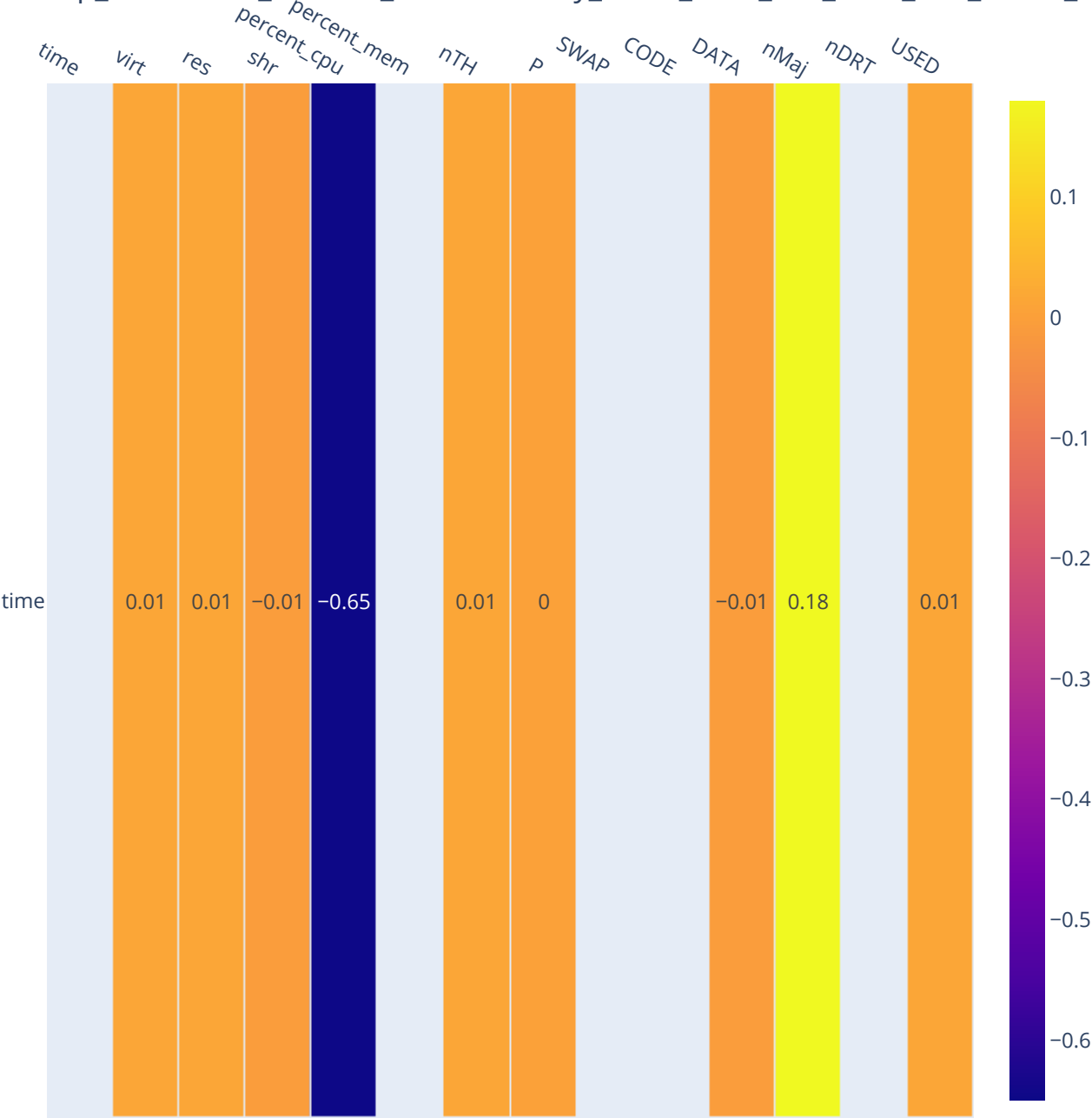
java - top_correlation_General_FilteredNbody_ONLY_1.8.0_382_9.0.4_and_10.0.2_Ver
