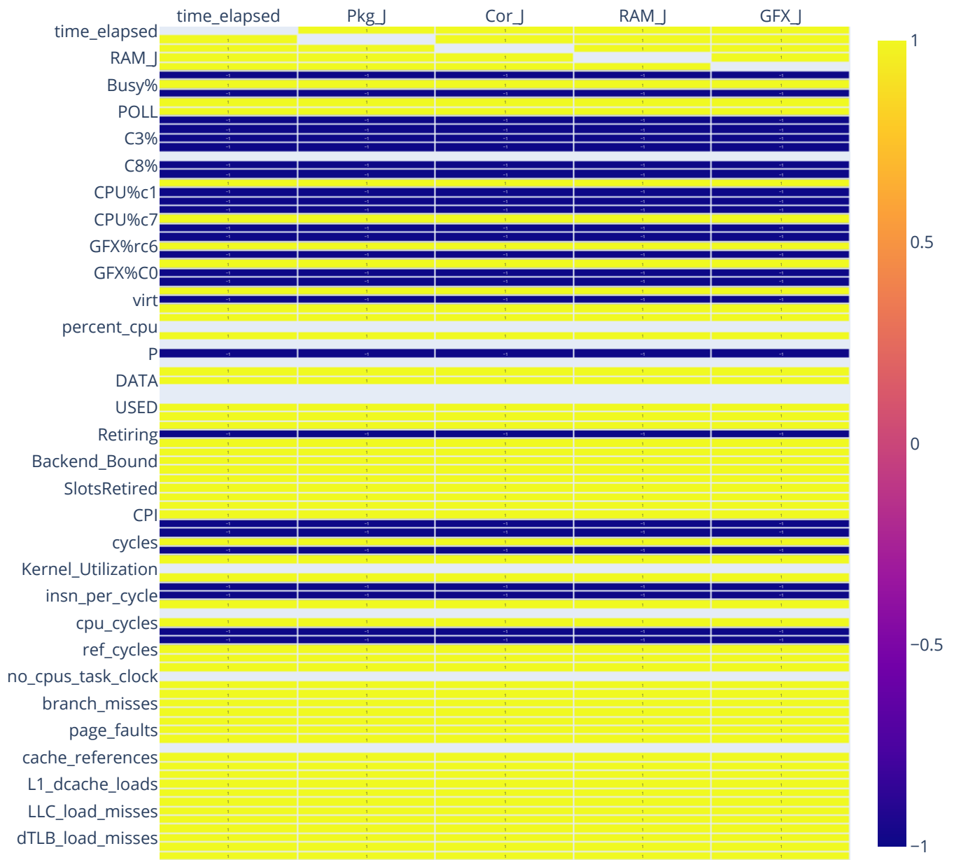
js - general_correlation_MedianValues_Filtered_ONLY_6.17.1_and_7.10.1_Versions_nb
