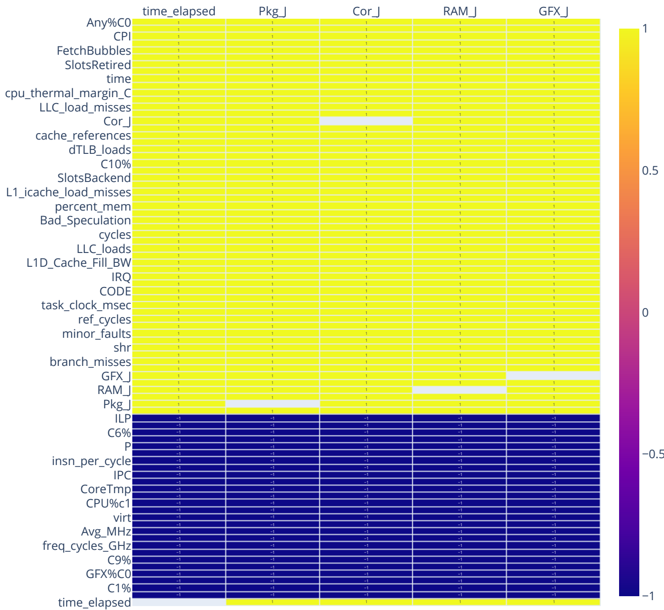
js - general_correlation_MedianValues_Filtered_ONLY_6.17.1_and_7.10.1_Versions_nb
