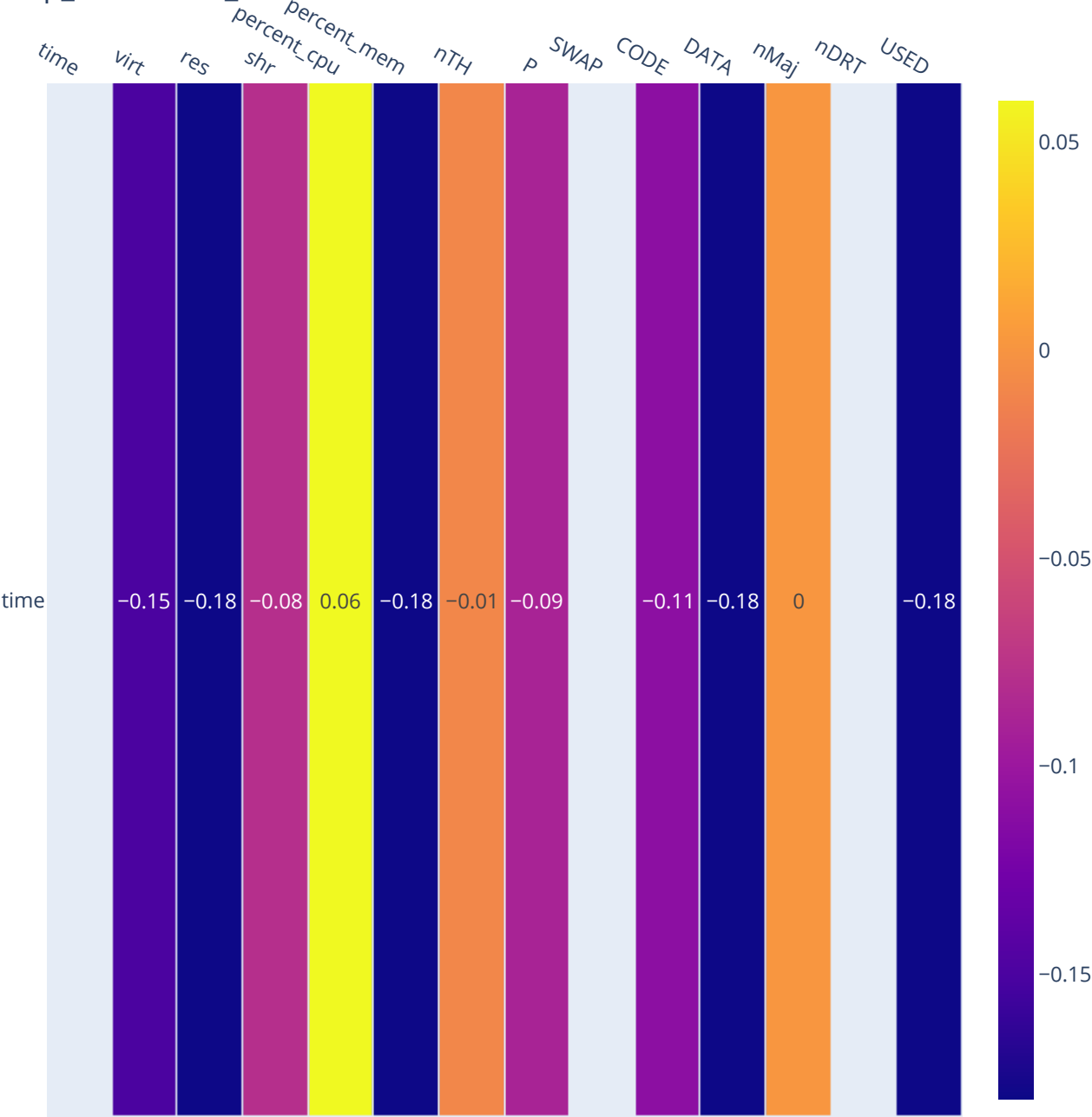
js - top_correlation_General
