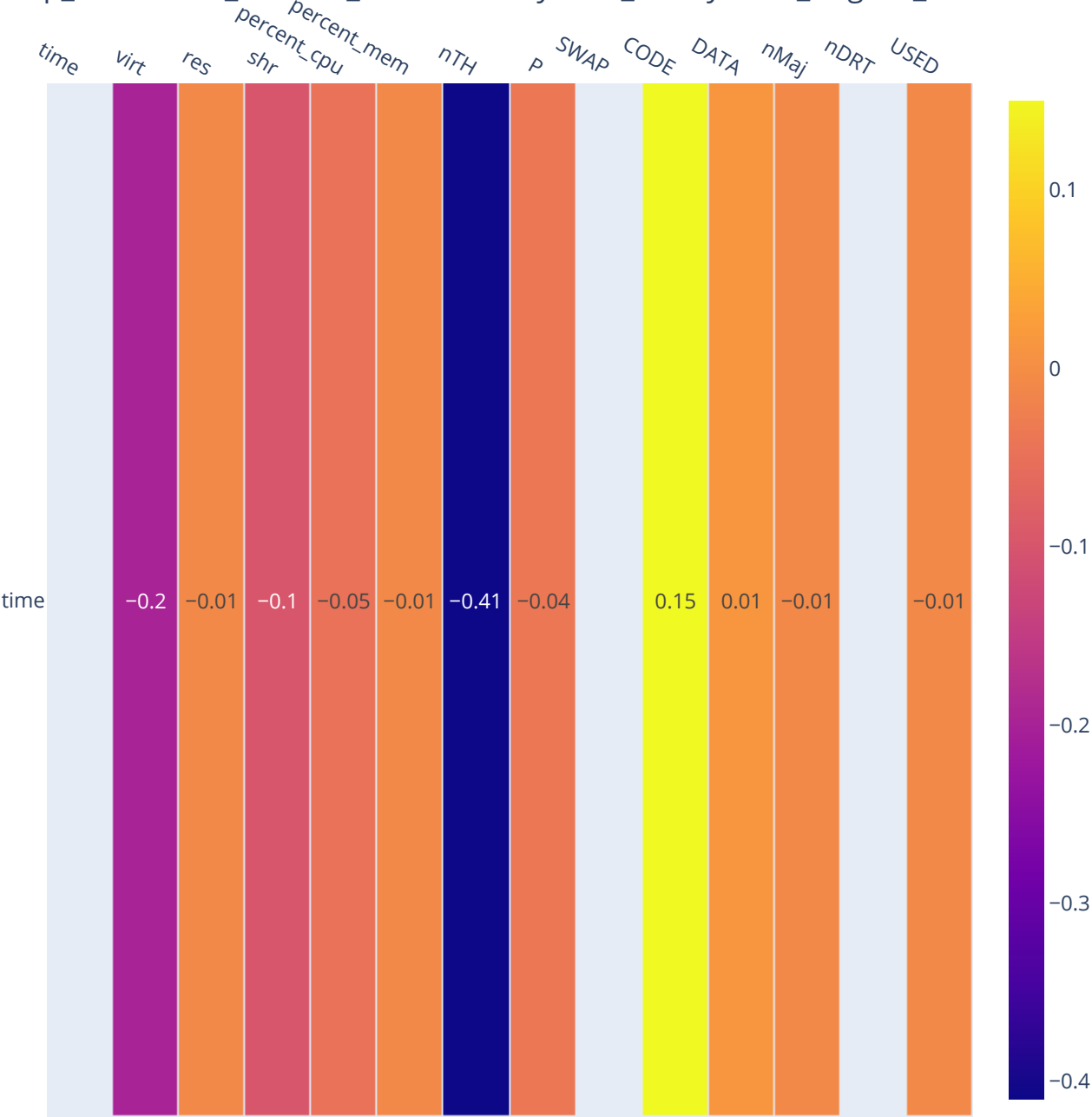
js - top_correlation_General_FilteredBinarytrees_binaryTrees_original_v1
