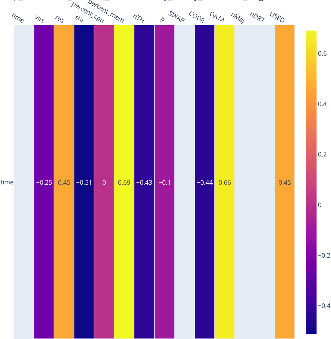
js - top_correlation_General_FilteredNbody_nbody_50000000_original
