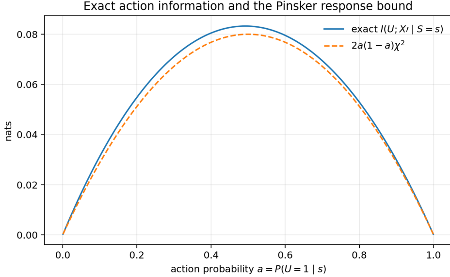
Figure 5: Example of Eq. (78) with p_0 = 0.25 and p_1 = 0.65 . The exact conditional mutual information lies above the Pinsker response term for every action probability. Both vanish when the policy almost never or almost always takes one action, illustrating the importance of action support.
