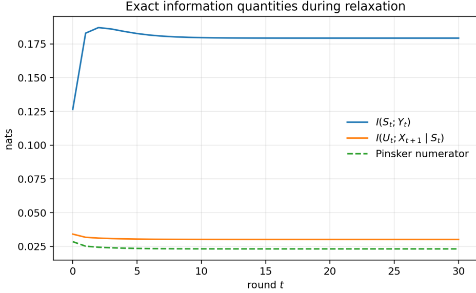
Figure 9: Exact sensing information, action-to-population CMI, and the Pinsker response numerator during relaxation of the reference model. The bound remains satisfied pointwise in time.
