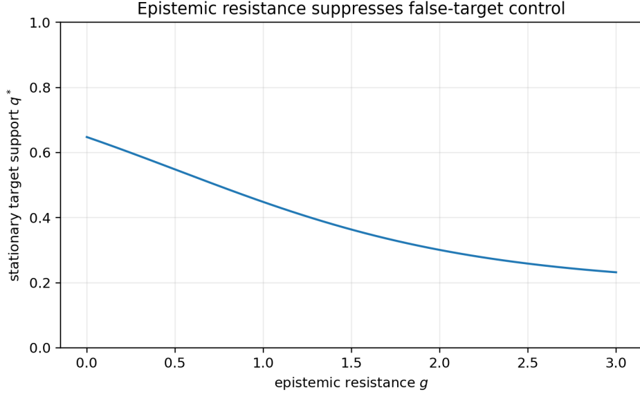
Figure 10: Exact stationary target support versus epistemic resistance. Increasing g shifts the controlled population away from the false controller target while leaving the autonomous K -process stationary fraction unchanged.
