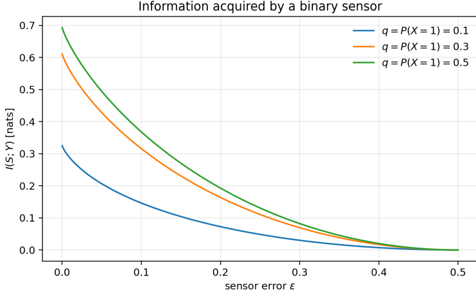
Figure 2: Exact sensing mutual information from Eq. (48). A balanced social state carries more potential information than a nearly deterministic social state, and all sensing information vanishes at \epsilon = 1/2 .
