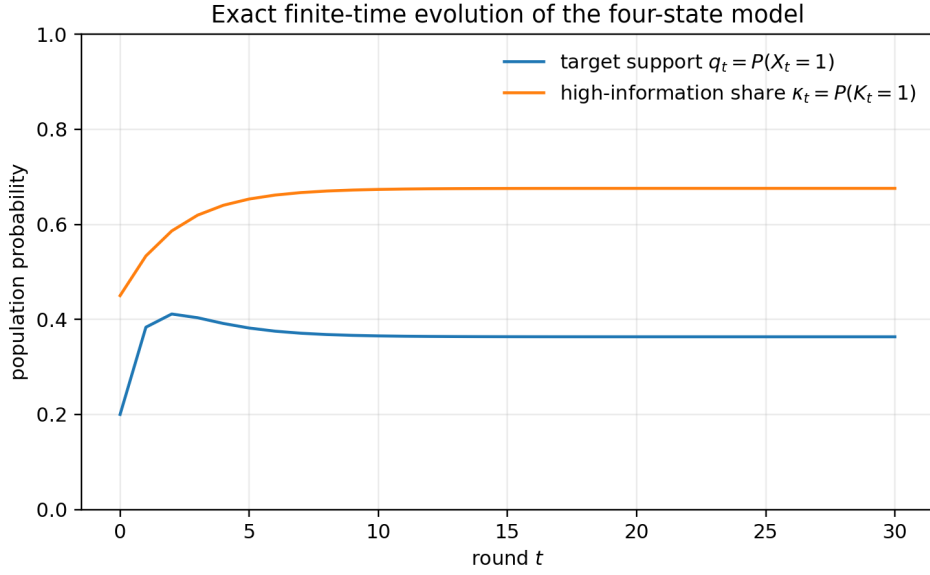
Figure 8: Exact finite-time population dynamics obtained from \mu_{t+1} = \mu_t M . No Monte Carlo sampling is used.
