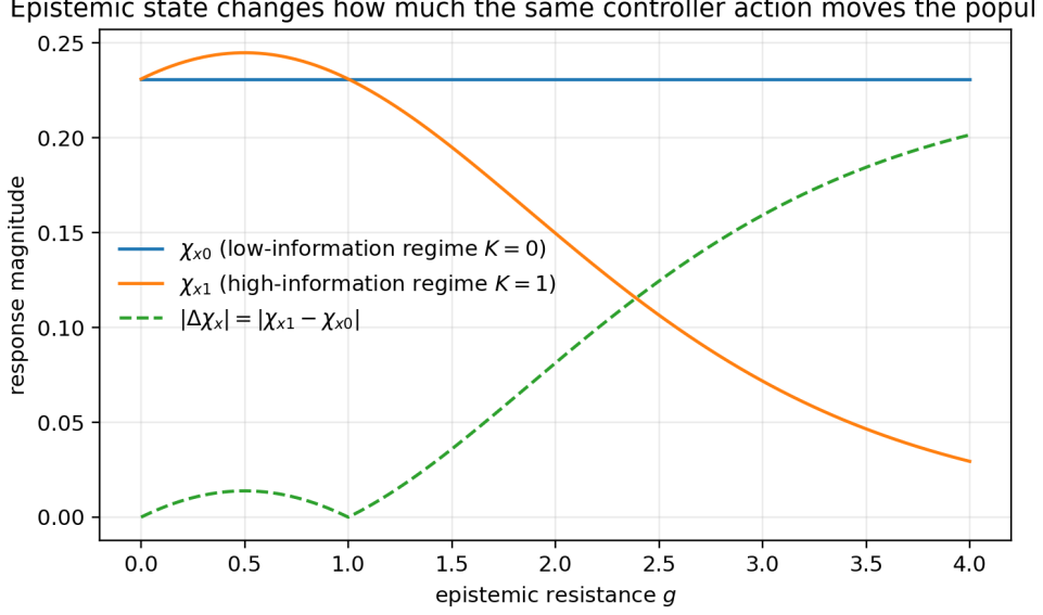
Figure 6: Epistemic modulation of local susceptibility for a fixed social state x = 0 . The low-information and high-information populations respond differently to the same intervention. The dashed curve shows the modulation gap |\Delta\chi_x| = |\chi_{x1} - \chi_{x0}| .
