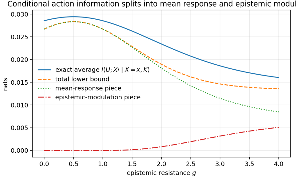
Figure 7: At a fixed social state x , the exact conditional action information (solid curve) exceeds the lower bound obtained by splitting the response into a mean-response contribution and an epistemic-modulation contribution. As epistemic resistance g increases, the controller affects low-information and high-information populations differently, and the modulation term grows.
