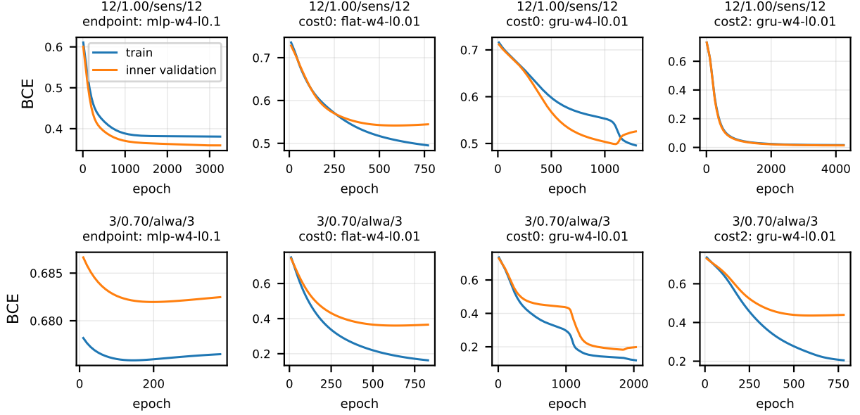
Figure 11: Training and inner-validation binary cross-entropy for neural candidates (outer fold 0, inner fold 0, seed 0, h = 10 ) in two comparisons. The GRU curves are still descending at the epoch cap.
