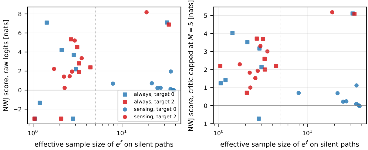
Figure 6: Weight concentration versus score at h = 10 . Left: raw NWJ; right: capped at M = 5 . The vertical line marks ESS = 5. Points with ESS \leq 5 have their objective dominated by a handful of silent paths.
