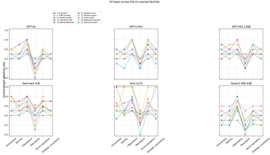
Figure 5: Per-task control-target adoption across the six families, one panel per model. The - Reputation trough appears in almost every task curve, but its depth is strongly task-dependent and a few task/model combinations invert the population-level ordering.
