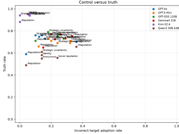
Figure 4: Truth rate against incorrect-target adoption rate, one point per model \times prompt family. Within each model the points spread horizontally — the framing moves susceptibility to a misleading controller — while truth rate varies far less, and the -Reputation points sit at the left edge with lower , not higher, truth rates.
