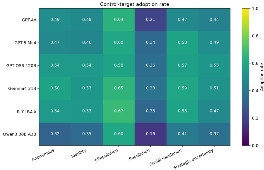
Figure 3: Control-target adoption rate for each model \times prompt family. The column structure is far more stable than the row structure: +Reputation is the brightest column for every model and -Reputation the darkest, while Anonymous and Identity are nearly indistinguishable.
