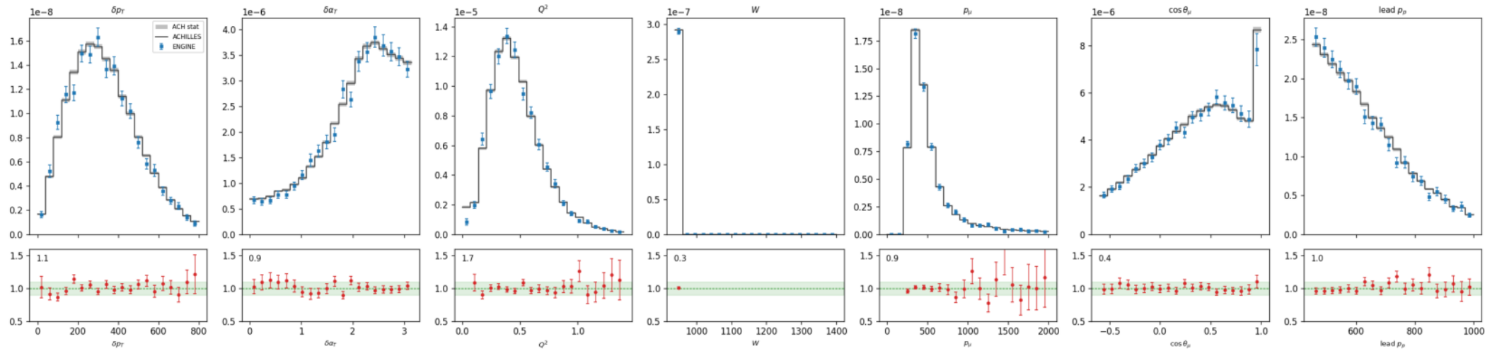
ArG cc0pi [qe] 2p FSI: ADONIS vs ACHILLES ACH/ADO 1.008
