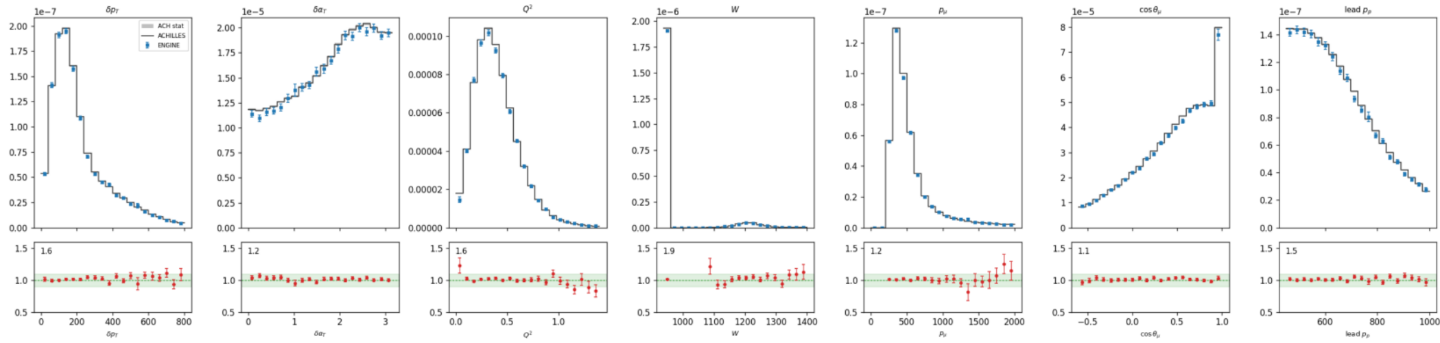
ArG cc0pi [both] incl FSI: ADoNIS vs ACHILLES ACH/ADO 1.016
