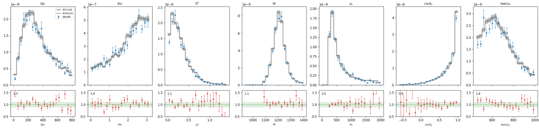
ArG cc0pi [res] 2p FSI: ADoNIS vs ACHILLES ACH/ADO 1.031
