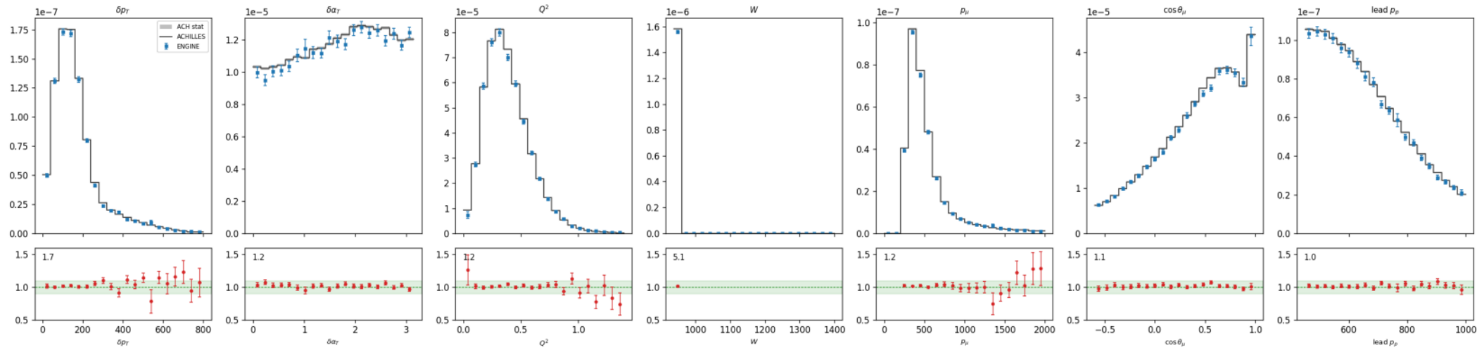
ArG cc0pi [qe] 1p FSI: ADONIS vs ACHILLES ACH/ADO 1.016
