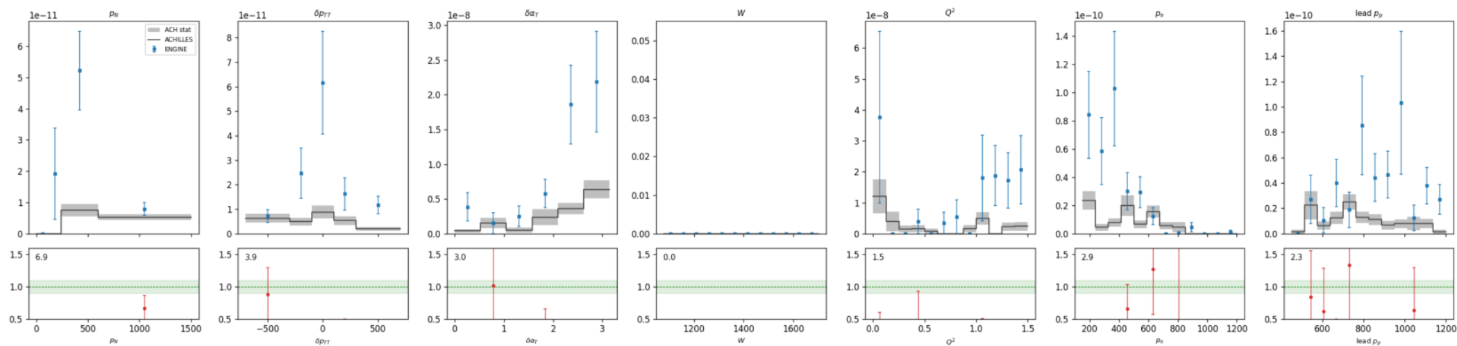
ArG cc1pi [qe] 2p FSI: ADoNIS vs ACHILLES ACH/ADO 0.274
