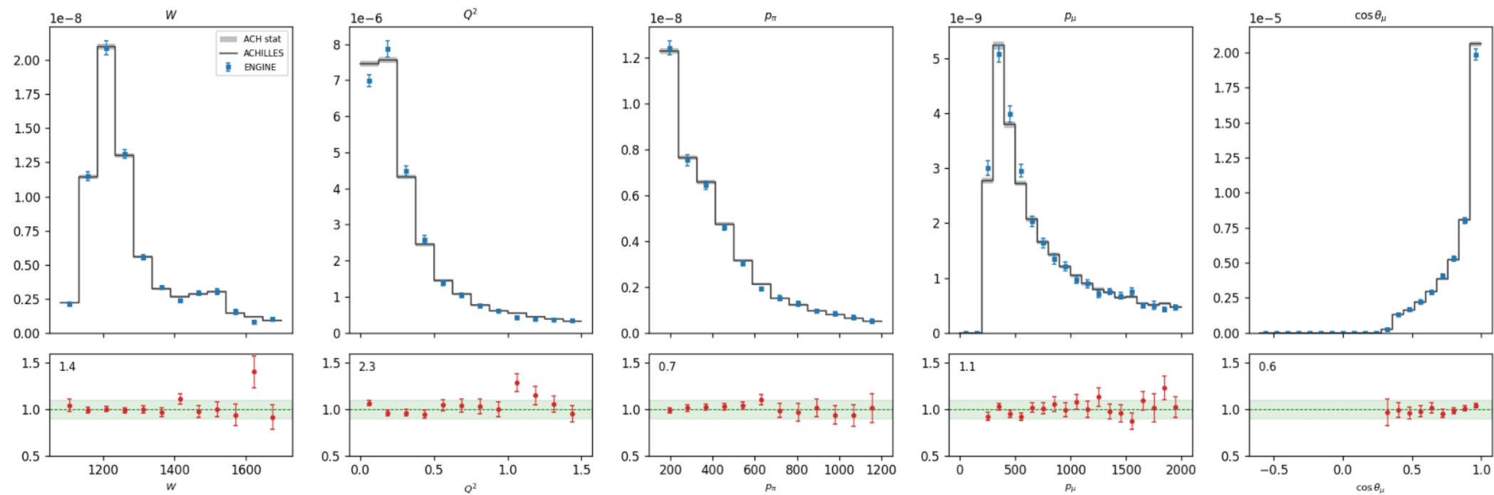
ArG cc1pi [both] 0p FSI: ADoNIS vs ACHILLES ACH/ADO 1.011
