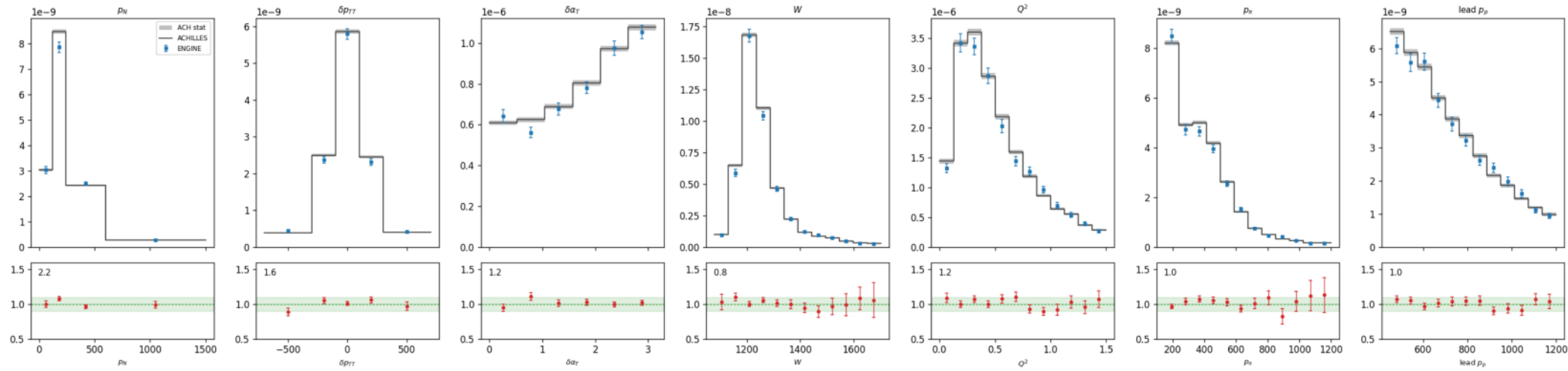
ArG cc1pi [both] incl FSI: ADONIS vs ACHILLES ACH/ADO 1.018
