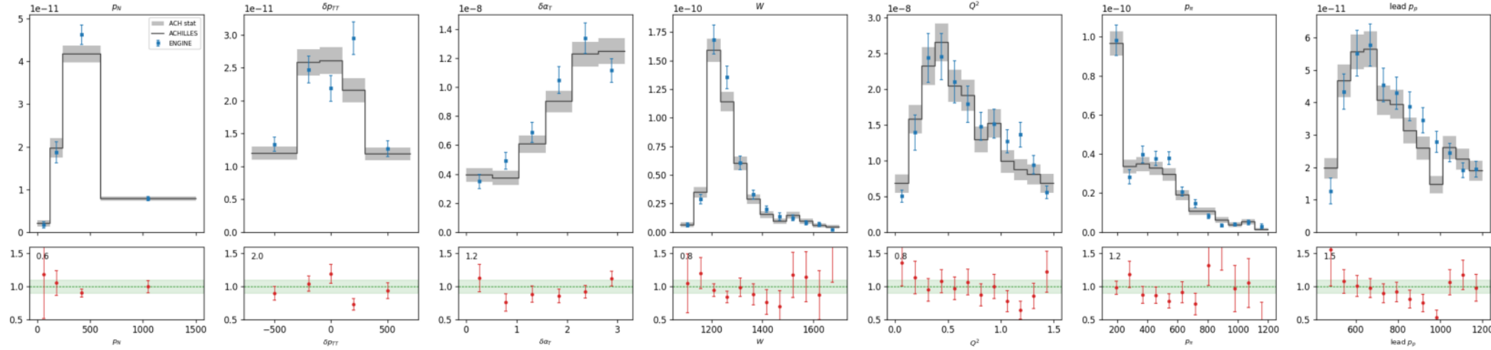
C cc1pi [res] 2p: ADoNIS vs ACHILLES ACH/ADO 0.945
