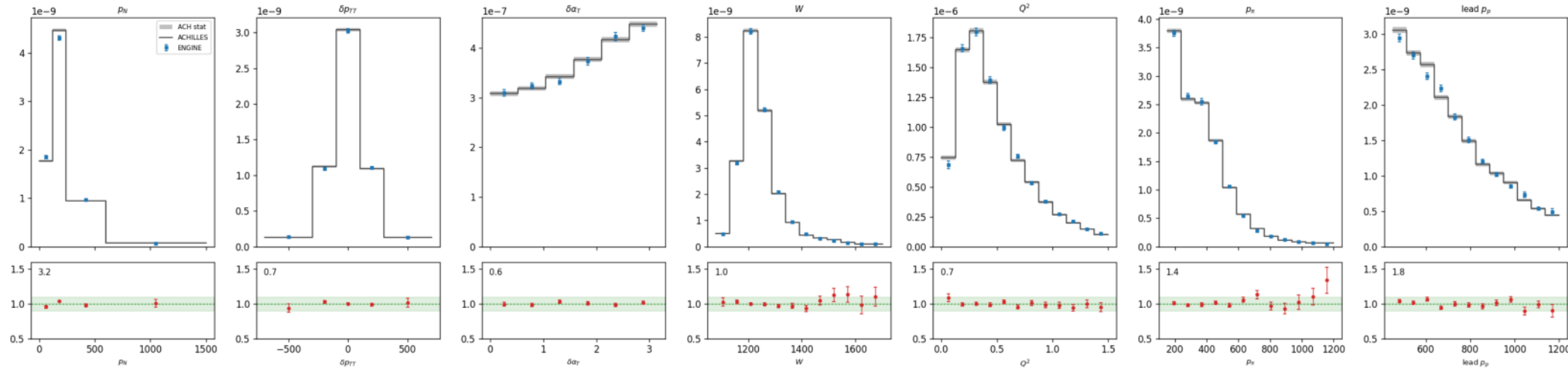
C cc1pi [both] 1p: ADoNIS vs ACHILLES ACH/ADO 1.004
