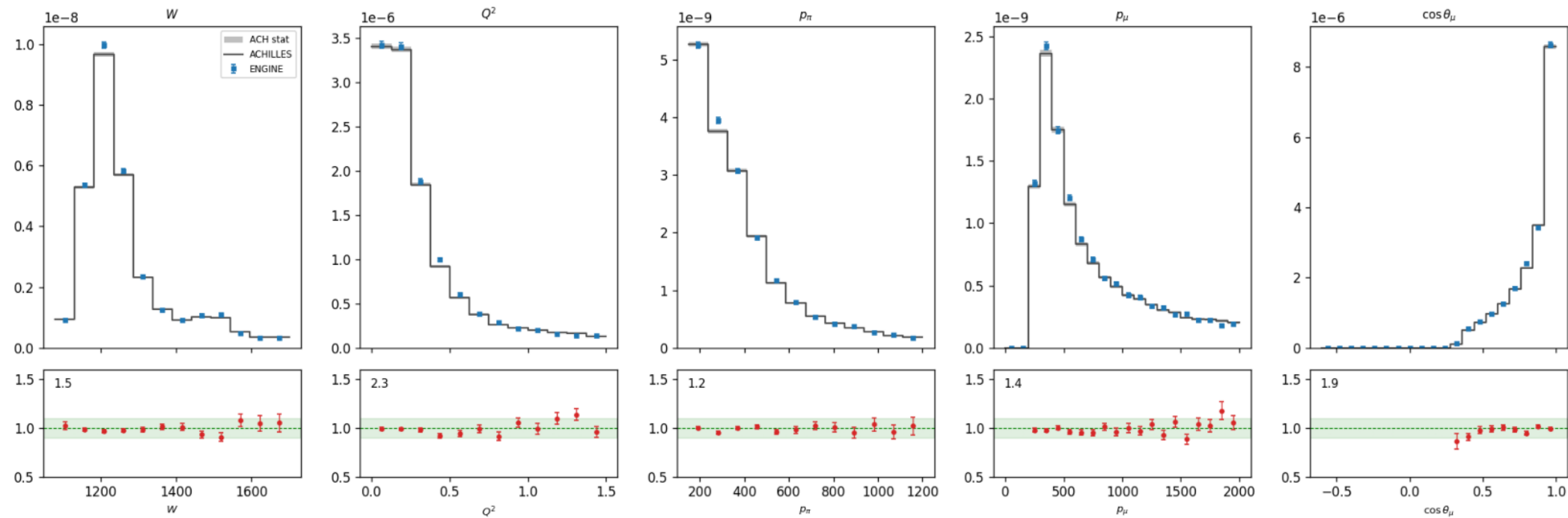
C cc1pi [both] 0p: ADoNIS vs ACHILLES ACH/ADO 0.990
