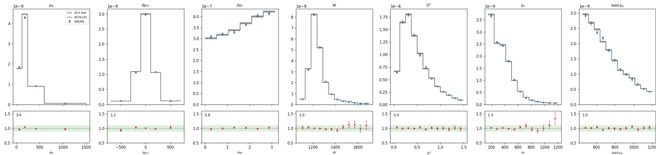
C cc1pi [res] 1p: ADoNIS vs ACHILLES ACH/ADO 1.004
