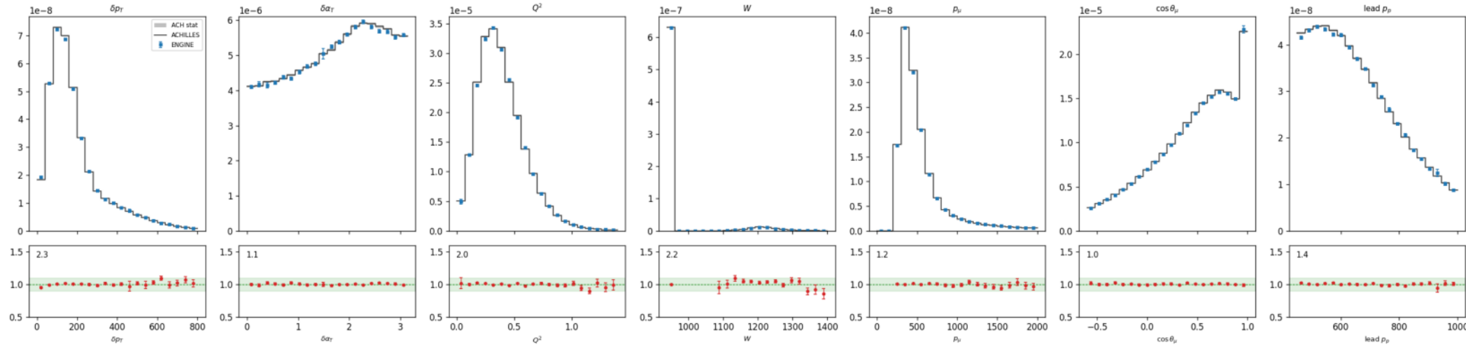
C cc0pi [both] incl: ADONIS vs ACHILLES ACH/ADO 1.005
