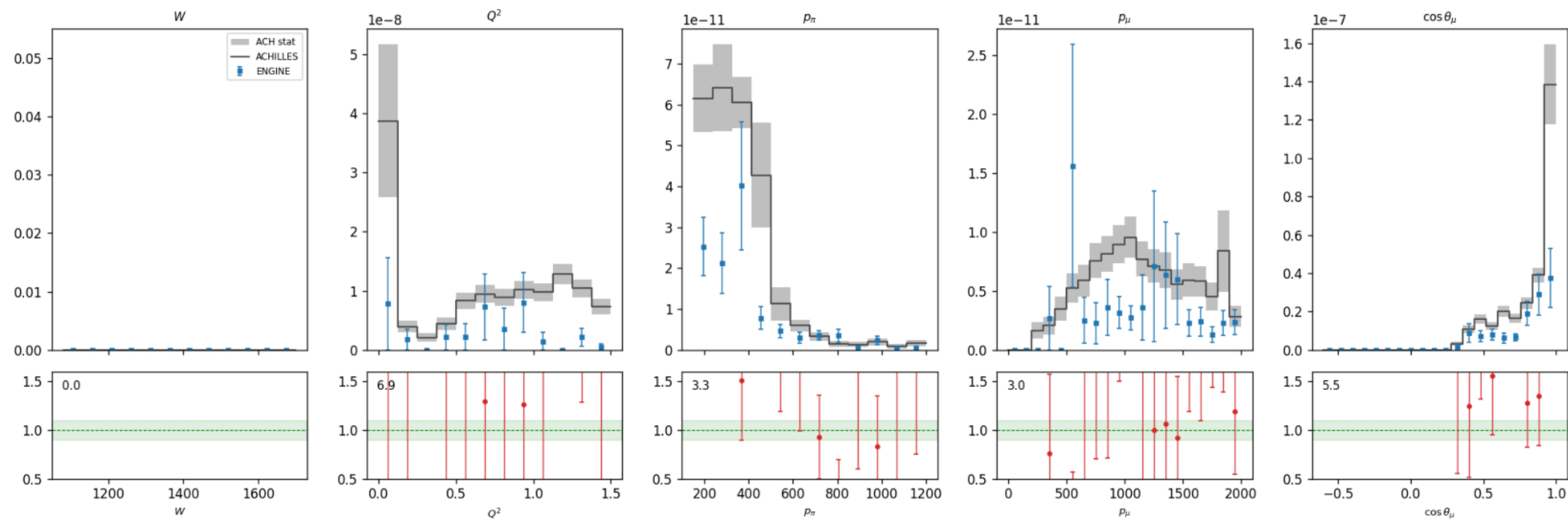
CG cc1pi [qe] 0p FSI: ADoNIS vs ACHILLES ACH/ADO 2.271
