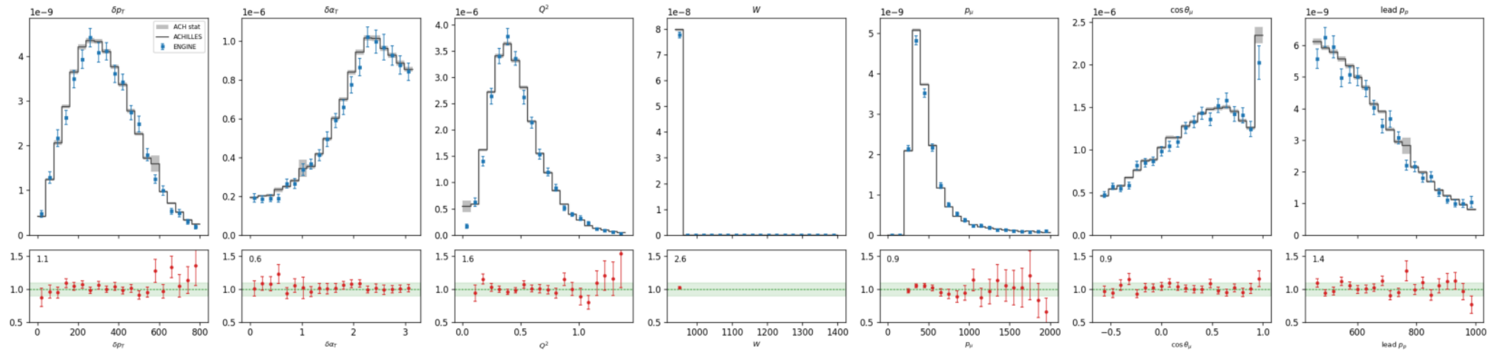
CG cc0pi [qe] 2p FSI: ADoNIS vs ACHILLES ACH/ADO 1.026
