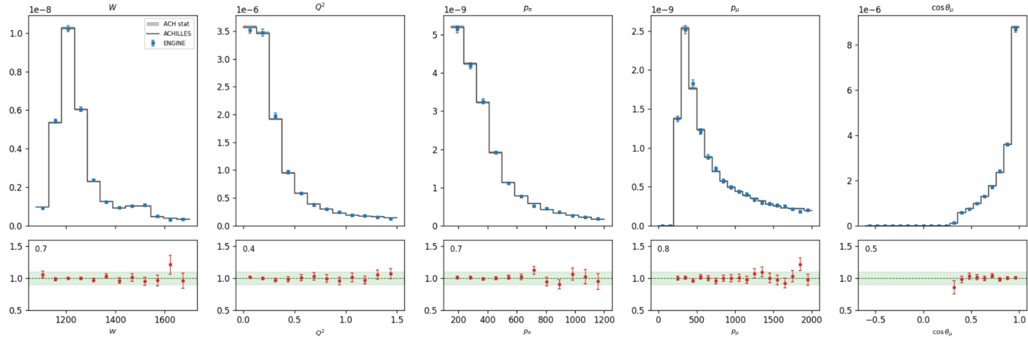
CG cc1pi [both] 0p FSI: ADONIS vs ACHILLES ACH/ADO 1.007
