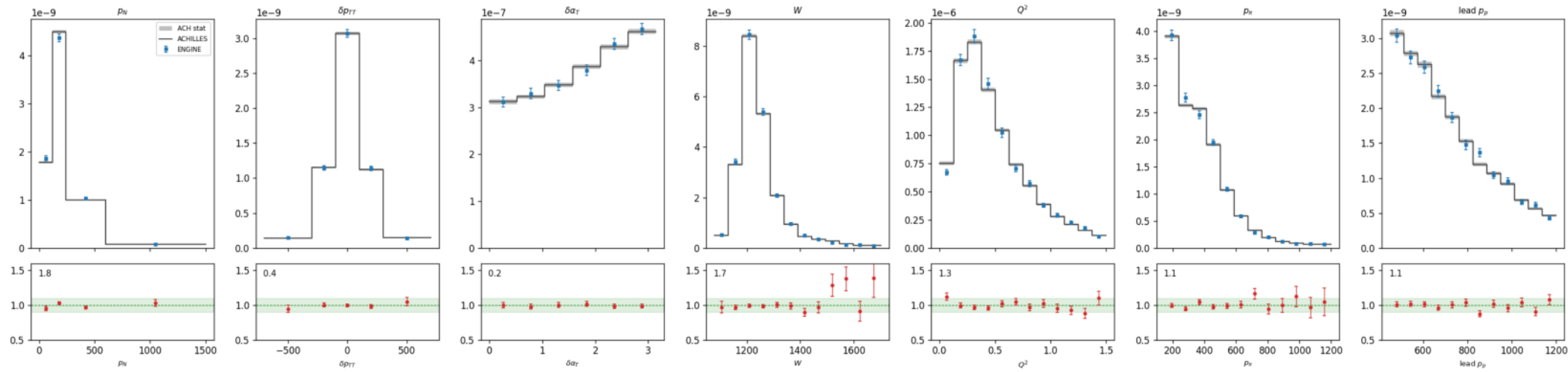
C cc1pi [both] incl FSI: ADoNIS vs ACHILLES ACH/ADO 0.996
