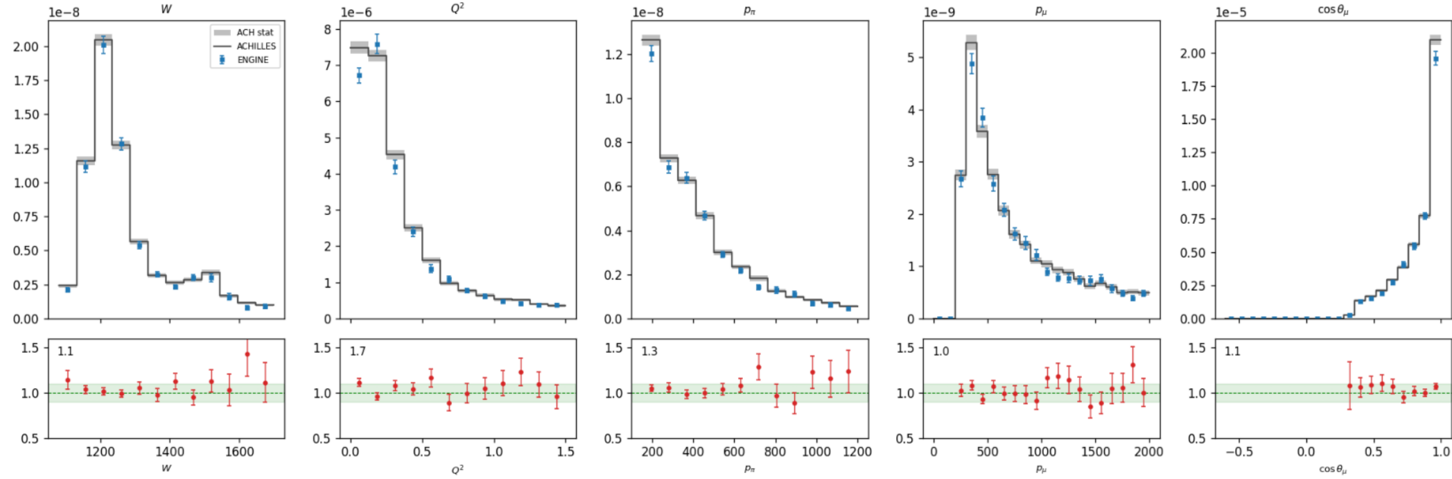
Ar cc1pi [both] 0p FSI: ADoNIS vs ACHILLES ACH/ADO 1.044
