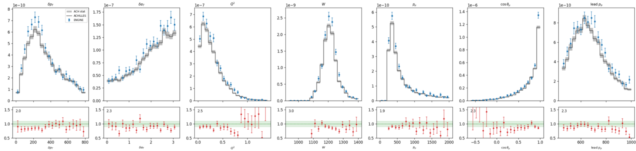
C cc0pi [res] 2p FSI: ADoNIS vs ACHILLES ACH/ADO 0.884
