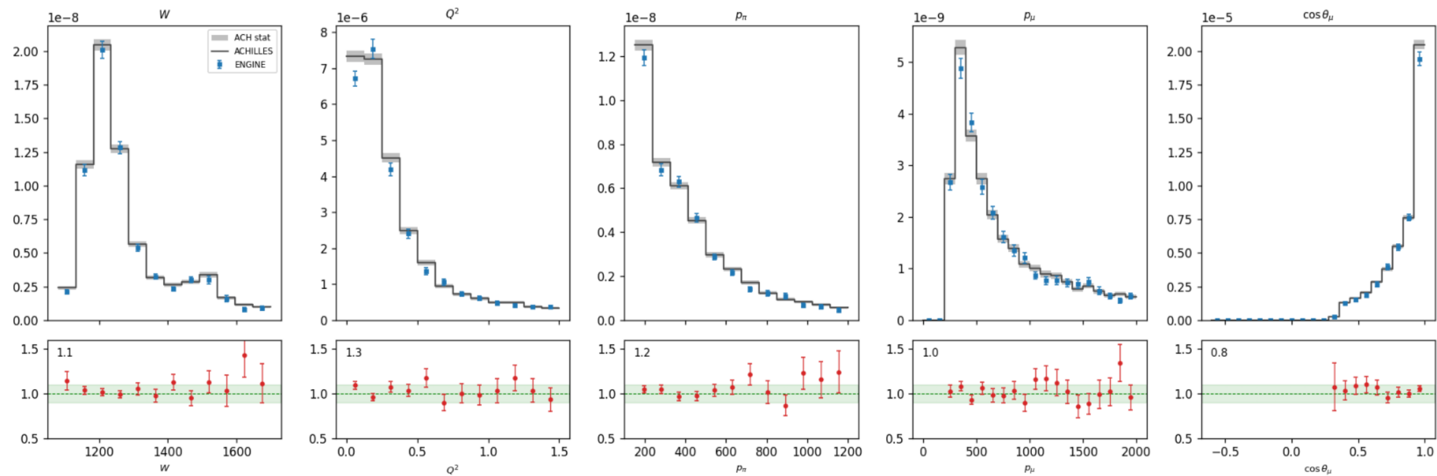
Ar cc1pi [res] 0p FSI: ADoNIS vs ACHILLES ACH/ADO 1.035
