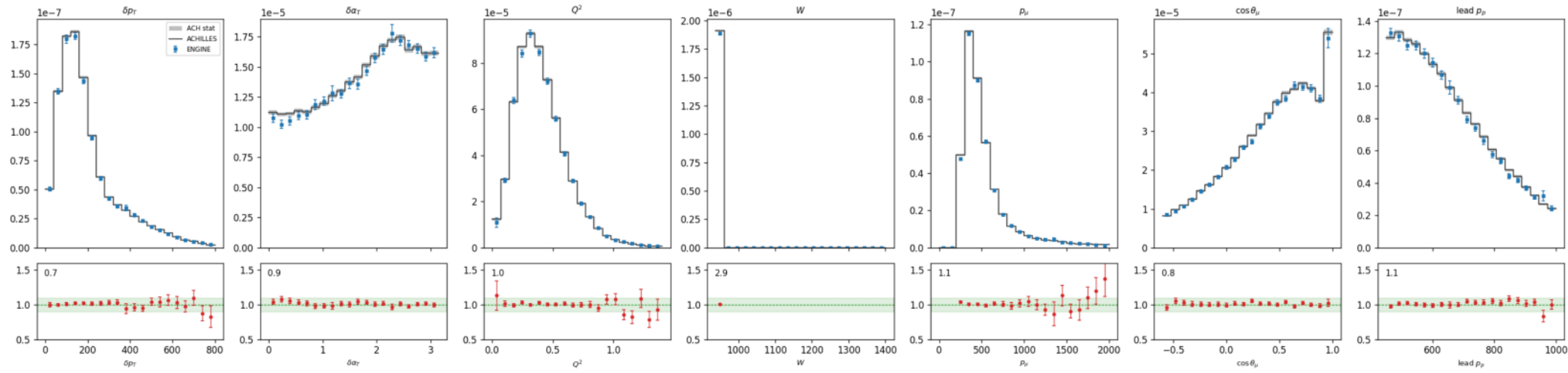
Ar cc0pi [qe] incl FSI: ADoNIS vs ACHILLES ACH/ADO 1.013
