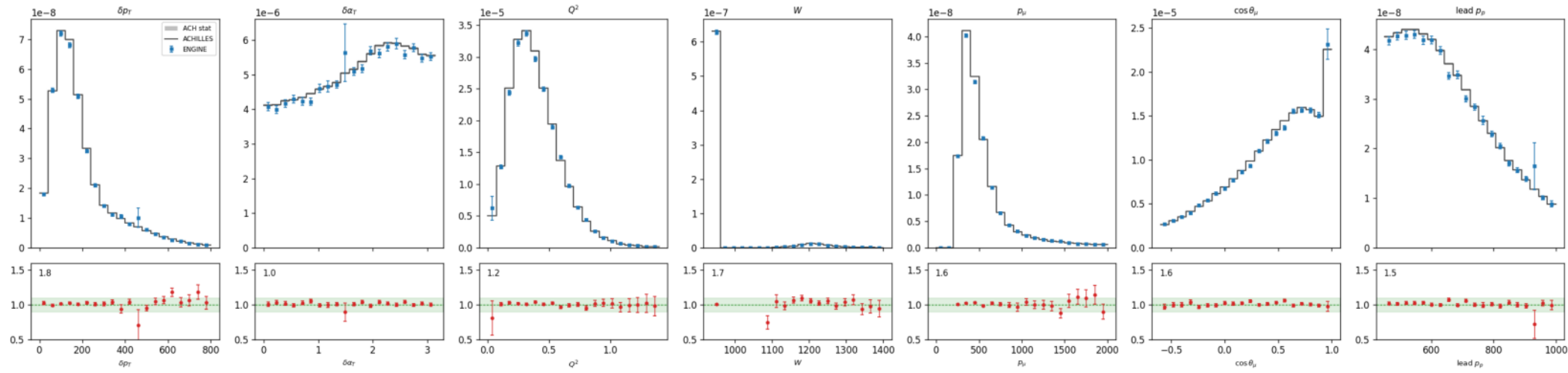
C cc0pi [both] incl FSI: ADoNIS vs ACHILLES ACH/ADO 1.009
