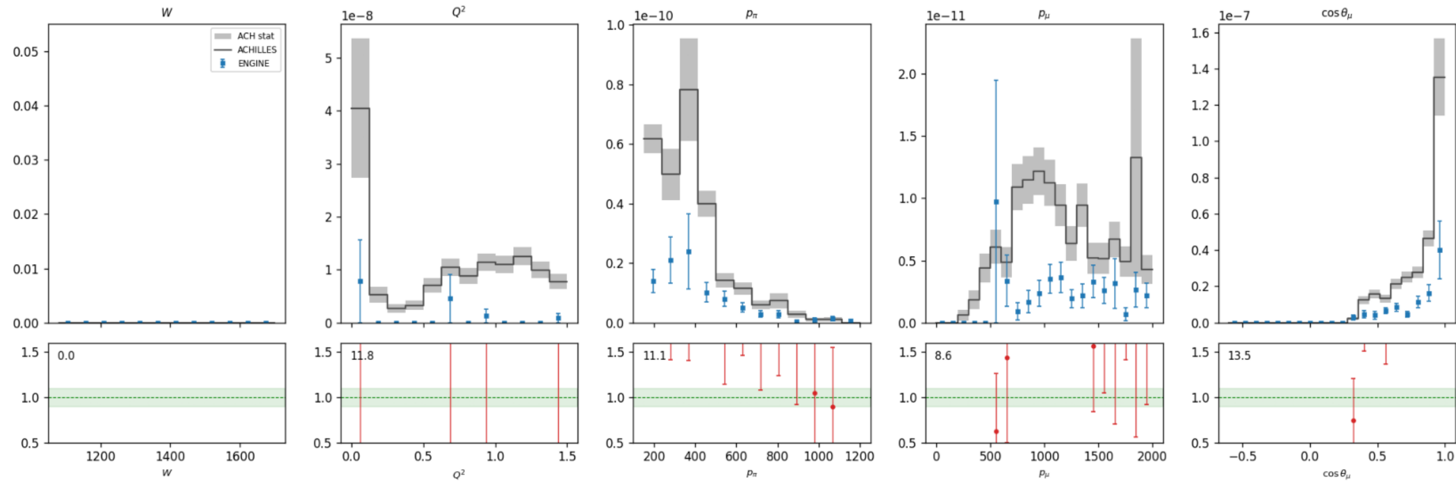
C cc1pi [qe] 0p FSI: ADoNIS vs ACHILLES ACH/ADO 2.996
