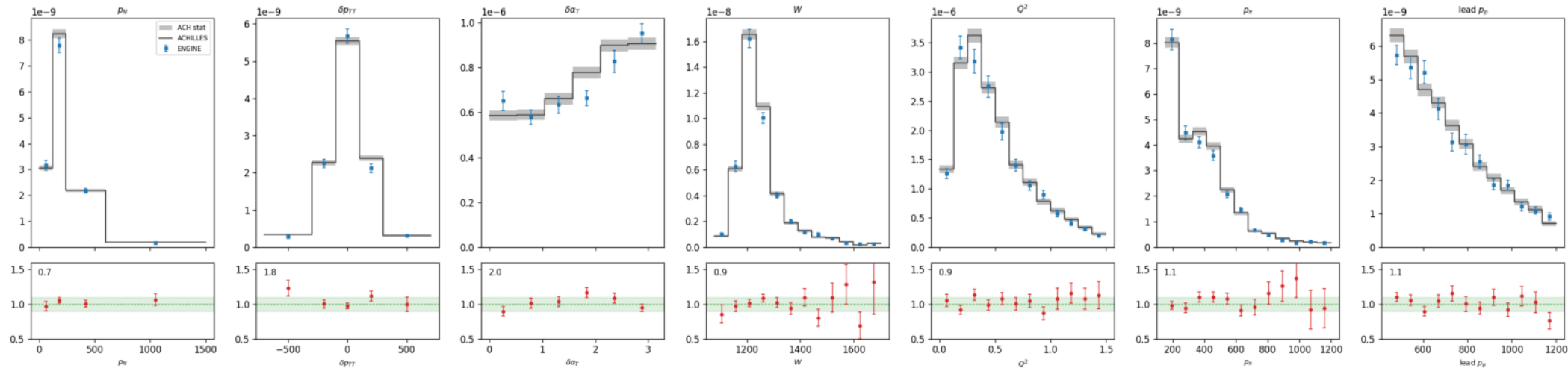
Ar cc1pi [res] 1p FSI: ADoNIS vs ACHILLES ACH/ADO 1.026
