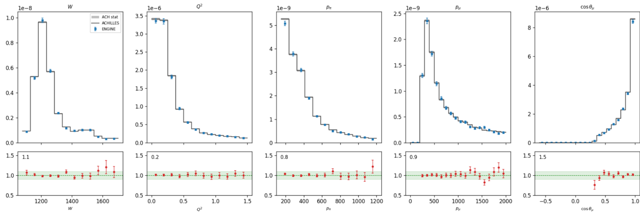
C cc1pi [both] 0p FSI: ADoNIS vs ACHILLES ACH/ADO 1.014
