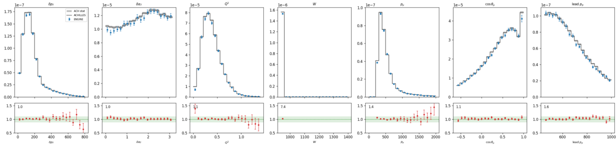
Ar cc0pi [qe] 1p FSI: ADoNIS vs ACHILLES ACH/ADO 1.021
