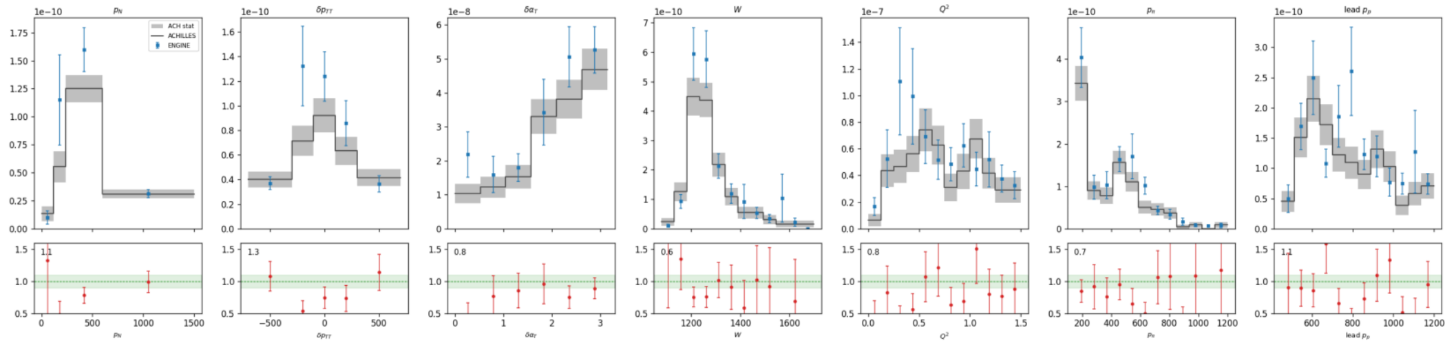
Ar cc1pi [res] 2p FSI: ADoNIS vs ACHILLES ACH/ADO 0.807
