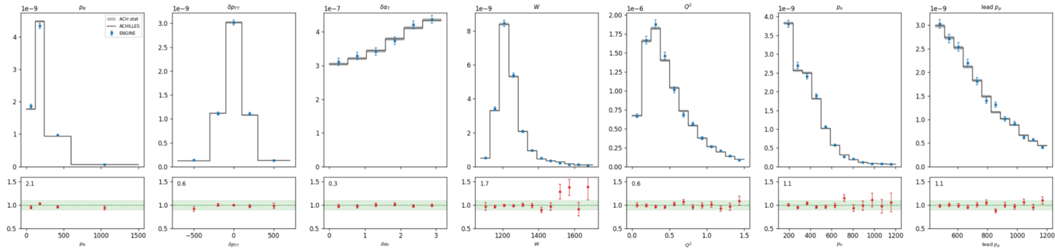
C cc1pi [res] incl FSI: ADoNIS vs ACHILLES ACH/ADO 0.991
