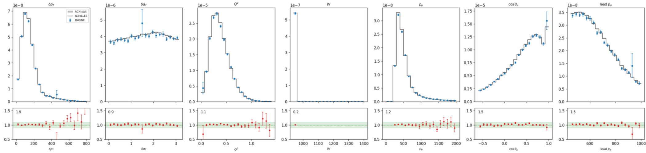
C cc0pi [qe] 1p FSI: ADoNIS vs ACHILLES ACH/ADO 1.005
