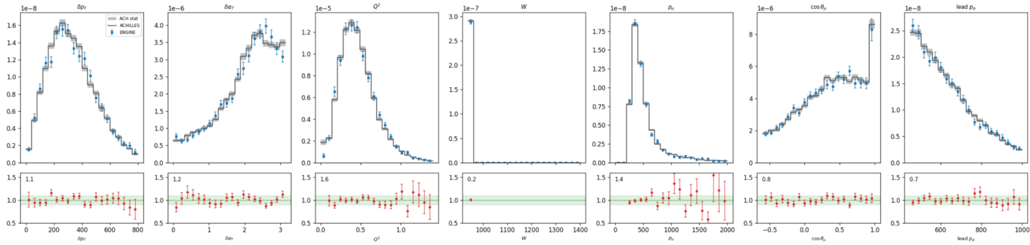
Ar cc0pi [qe] 2p FSI: ADoNIS vs ACHILLES ACH/ADO 1.007
