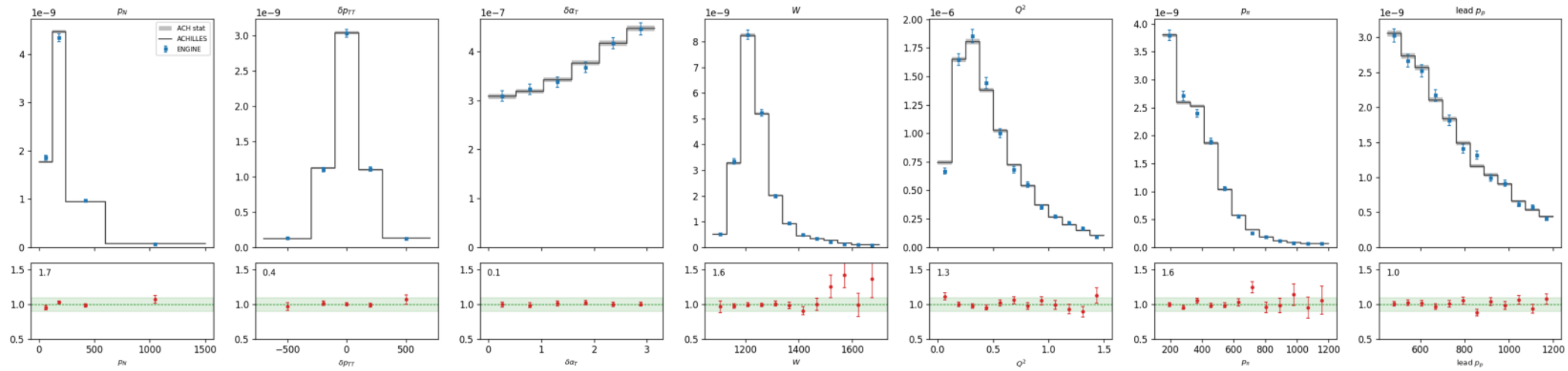
C cc1pi [both] 1p FSI: ADoNIS vs ACHILLES ACH/ADO 1.004
