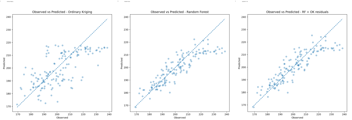
Figure 2. Observed versus predicted values for the synthetic test set. A , Ordinary Kriging produces predictions that are compressed toward a narrower range, reflecting the smoothing effect of spatial averaging under a stationary covariance model. B , Random Forest captures more of the nonlinear covariate-driven signal, so the points follow the identity line more closely, although residual dispersion remains. C , The hybrid RF + OK residual model gives the strongest agreement between observations and predictions because it combines nonlinear covariate learning with explicit modeling of residual spatial dependence. Overall, the panel shows why hybrid spatial workflows [63] can outperform either geostatistics [30] or machine learning [76] alone when the target field contains both deterministic environmental structure and spatially correlated residual variation [43].
