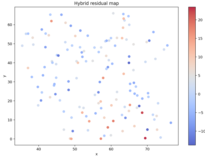
Figure 3. Spatial residuals from the hybrid RF + OK residual model. Warm and cool colors identify local overprediction and underprediction after combining nonlinear covariate learning with residual kriging.
