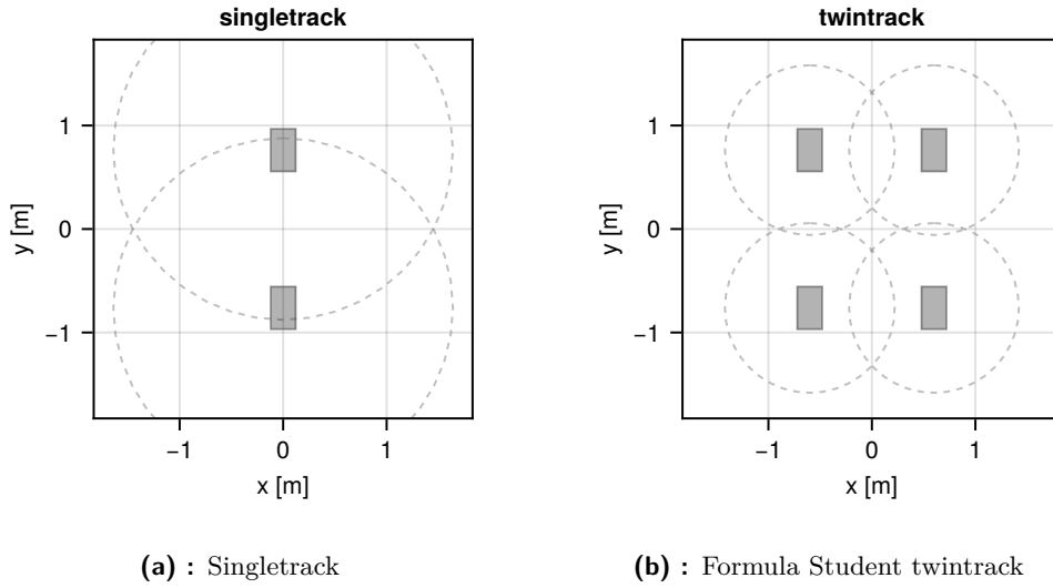
Figure 6.9: Single-track and Formula Student twintrack vehicle models.
