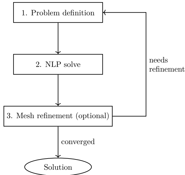
Figure 5.1: Optimal control problem solving pipeline. Adapted from [14, p. 91]
