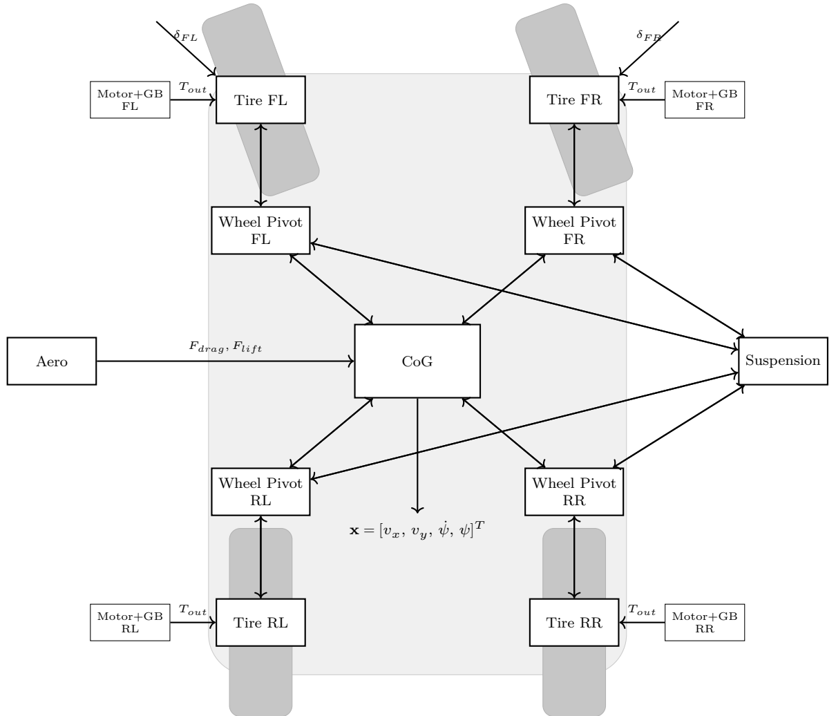
Figure 2.10: Twin-track model
