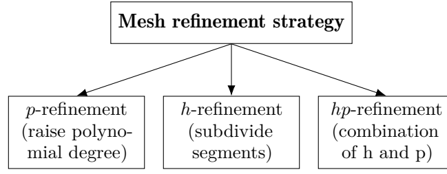
Figure 3.6: Mesh refinement categories [22, 56].
