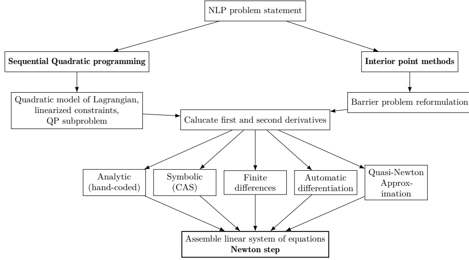
Figure 4.2: NLP solution flow: problem statement → solver family (SQP / IPM) → derivative computation → assembled Newton step.
