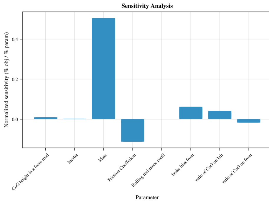
Figure 6.2: Sensitivity of lap time to vehicle parameters.
