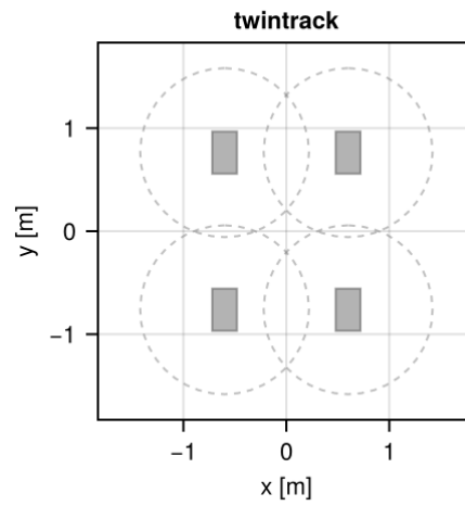
Figure 6.10: Formula Student twintrack vehicle model.
