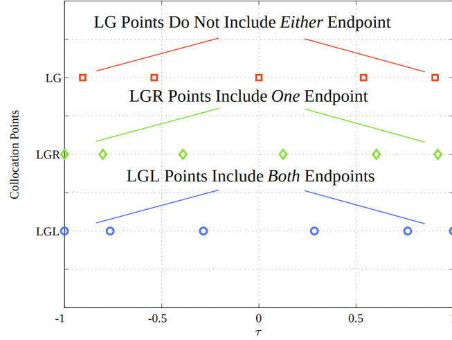
Figure 3.5: Schematic Showing the Differences Between LGL, LGR, and LG Collocation Points, taken from [26]
