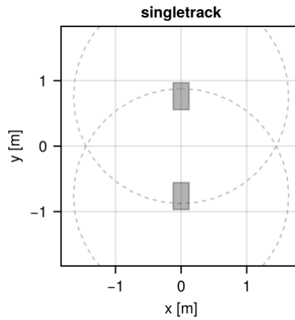
Figure 6.9: Singletrack vehicle model.
