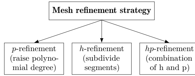
Figure 3.6: Mesh refinement categories [21, 55].
