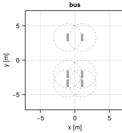
Figure 6.12: Bus vehicle model.
