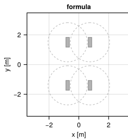
Figure 6.11: Formula E vehicle model.
