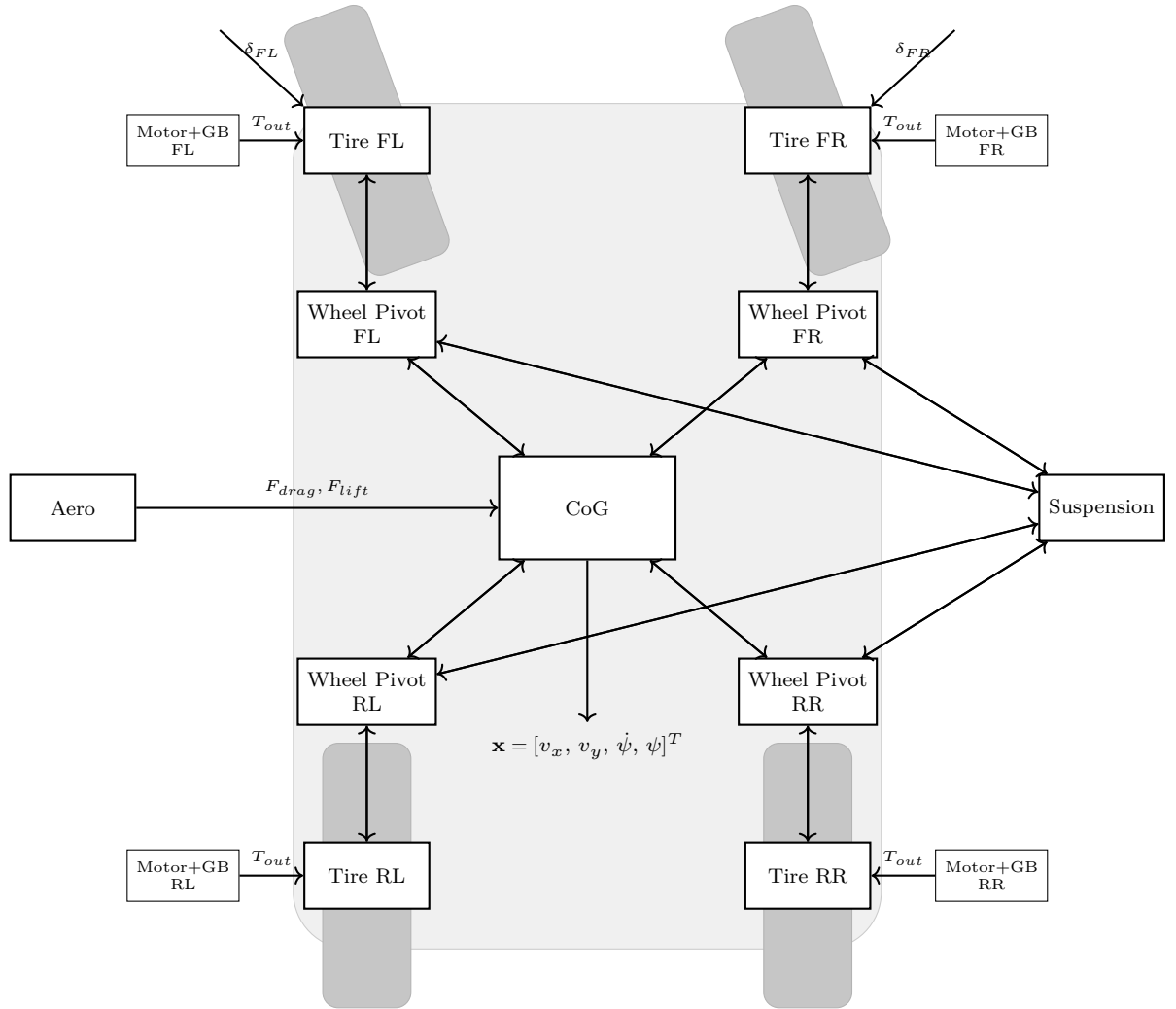
Figure 2.10: Twin-track model
