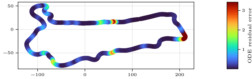
Figure 3.7: Node-interval ODE error for power-test case.
