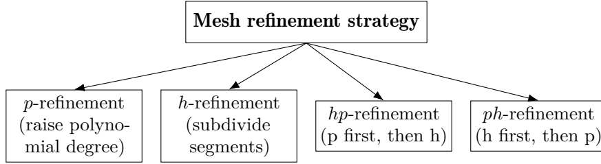
Figure 3.5: Mesh refinement [20, 48].
