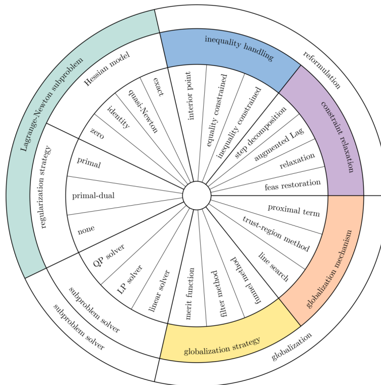
Figure 4.1: Unifying framework: the “wheel of strategies”[?]
