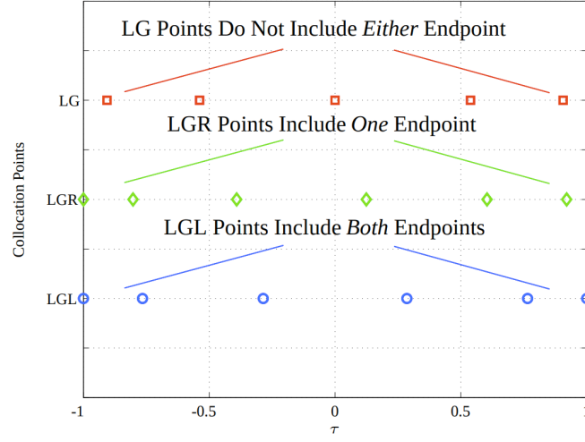
Figure 3.5: Schematic Showing the Differences Between LGL, LGR, and LG Collocation Points, taken from [?]
