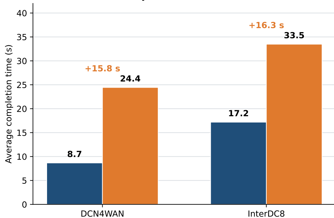
(b) AllGather completion
