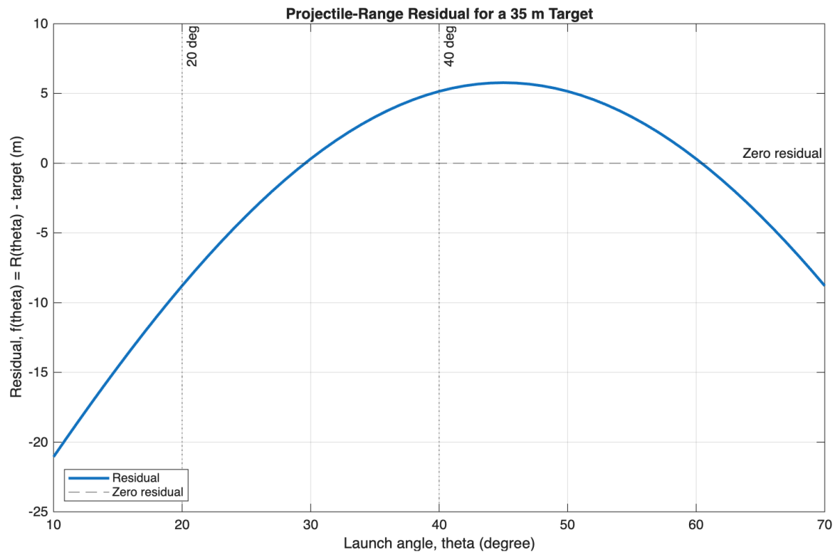
Figure 1: MATLAB-generated residual graph for the locked projectile model. The selected low-angle bracket from 20^\circ to 40^\circ contains a sign change.
