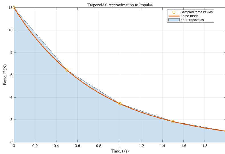
Figure 1: Week 7 force-time model: five samples define four trapezoids whose total area estimates the impulse.
