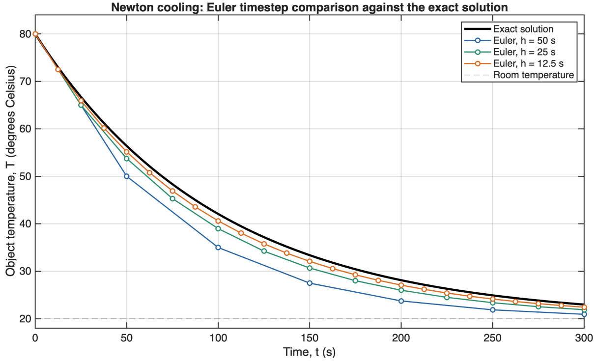
Figure 1: Newton cooling from 80^{\circ}\text{C} toward a 20^{\circ}\text{C} environment. Euler trajectories use h = 50, 25 , and 12.5\text{s} ; the black line is the supplied exact reference.
