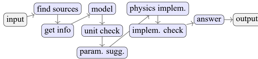
Figure 2: Overview of all the Tasks and their order as they are performed by the Physics Modelling Assistant. The system receives an input string as a free form modelling request; it will find papers on that topic and download them from arXiv; the papers will be read and necessary information gets extracted; a model is build based on the extracted information; the formulas of the model are checked for unit consistency; realistic starting parameters are suggested for the simulation; the model is implemented into Python code; the code is checked and corrected if necessary; a final answer to the input is provided; output is the final answer and the files created by the individual tasks
