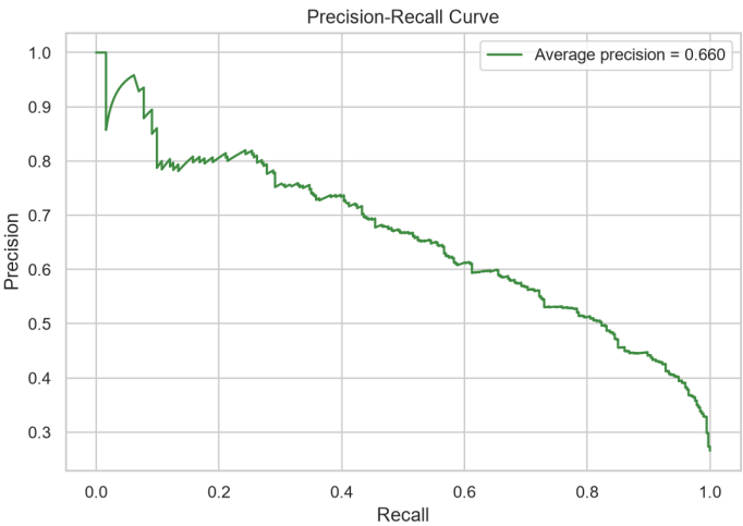
Precision-recall curve for selected model
