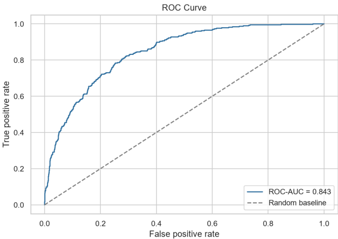
ROC curve for selected model
