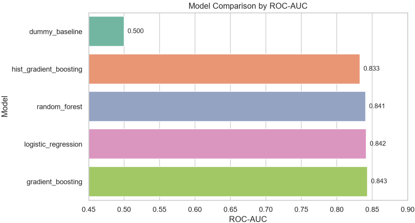
ROC-AUC comparison across trained models
