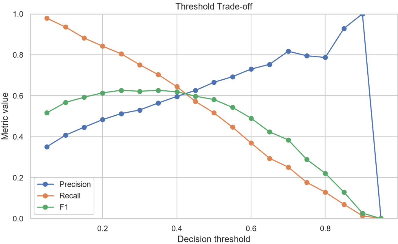
Precision, recall, and F1 across decision thresholds
