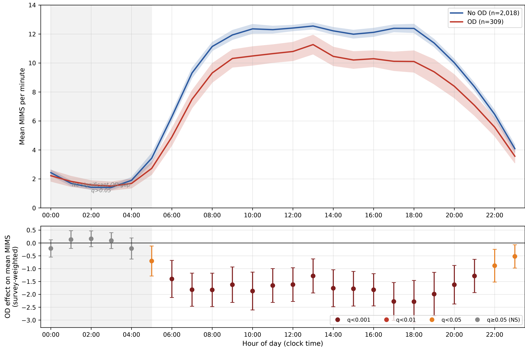
Figure S1. Hour-by-hour OD-non-OD activity gap with FDR significance (top: 24-hour profile; bottom: hourly OD effect with BH-FDR across 24 tests)
