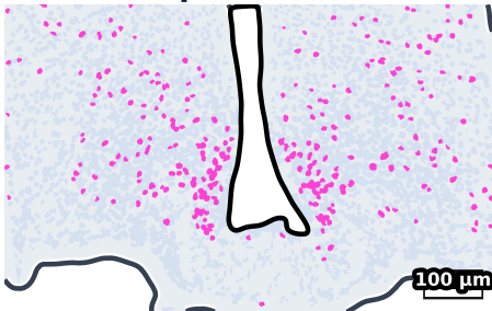
c-FOS-positive nuclei
