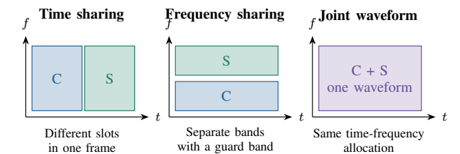
Fig. 3. Three conceptual time-frequency allocations. The axes t and f denote time and frequency. C and S denote communication and sensing use of a resource. A joint waveform reuses an allocation for both functions, whereas time and frequency sharing separate their allocations. The rectangles indicate the time-frequency resources assigned to each function, rather than measured spectra or performance.
