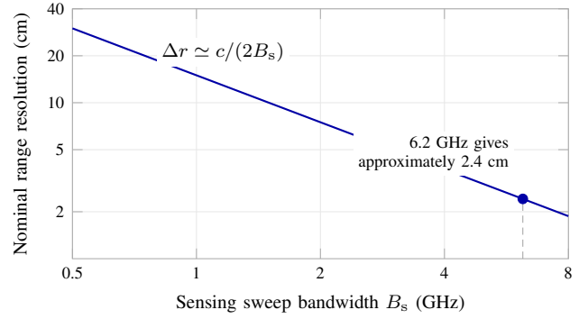
Fig. 4. Calculated nominal range resolution for an ideal two-way, bandwidth-limited measurement in air. The curve uses \Delta r = c/(2B_s) . The marked 6.2 GHz sweep corresponds to approximately 2.4 cm, as reported for the waveform in [10]. The calculation describes the nominal separation scale for two targets.
