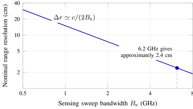
Fig. 4. Calculated nominal range resolution for an ideal two-way, bandwidth-limited measurement in air. The curve uses \Delta r \simeq c/(2B_s) . The marked 6.2 GHz sweep corresponds to approximately 2.4 cm, as reported for the waveform in [10]. The calculation describes the nominal separation scale for two targets.
