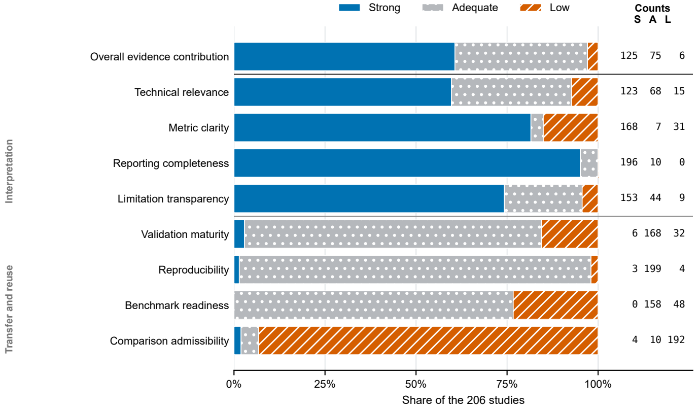
Fig. 8. Technical appraisal of the 206 included studies under the review-specific TQAF rules. Each row groups all studies by strong, adequate, or low support. The interpretation dimensions concern the meaning and reporting of results in their source setting. Transfer and reuse dimensions concern validation and reconstruction, together with benchmark and comparison support. Overall evidence contribution is displayed separately.
