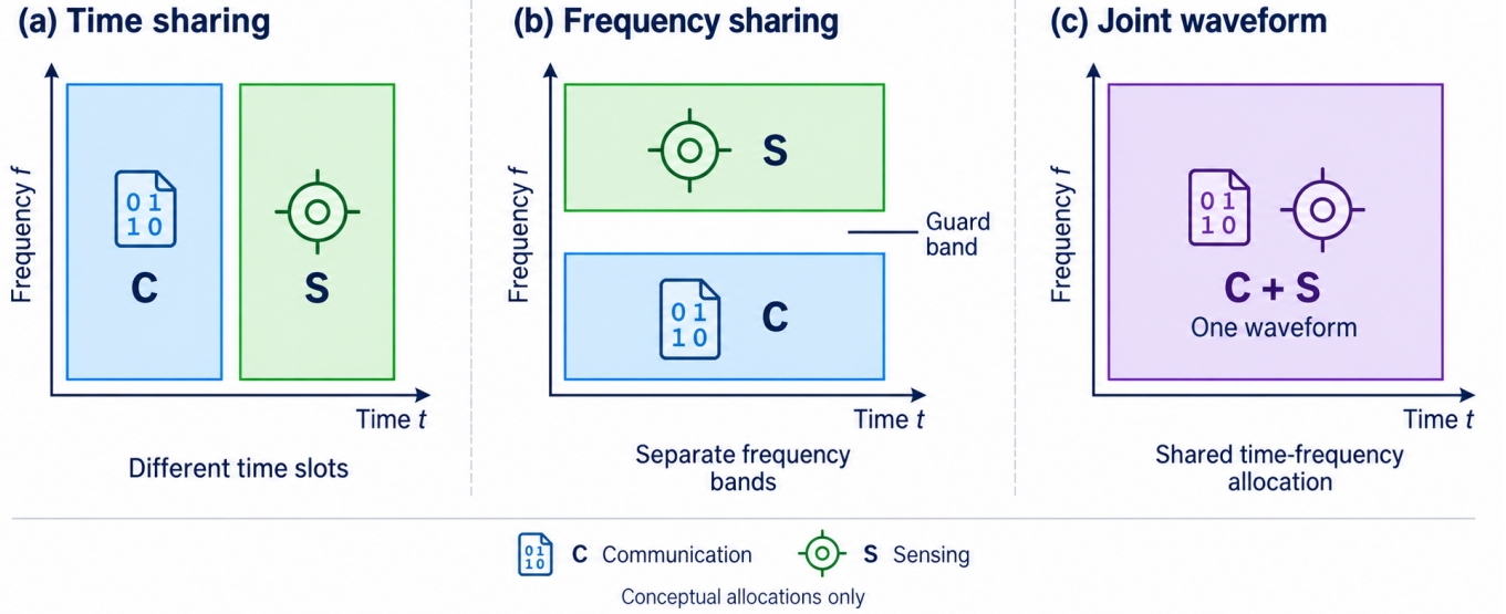
Fig. 4. Conceptual time-frequency allocations for communication and sensing. Panel (a) assigns different time slots to the two functions. Panel (b) assigns separate frequency bands, with a guard band shown in this example. Panel (c) uses one waveform within a shared allocation. The axes t and f denote time and frequency, and C and S denote communication and sensing. Icons identify the functions, while rectangles indicate allocated resources. Equal panel dimensions serve the illustration and do not assert equal bandwidth or performance.
