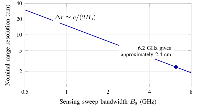
Fig. 5. Calculated nominal range resolution for an ideal two-way, bandwidth-limited measurement in air. The curve uses \Delta r = c/(2B_s) . The marked 6.2 GHz sweep corresponds to approximately 2.4 cm, as reported for the waveform in [10]. The calculation describes the nominal separation scale for two targets.
