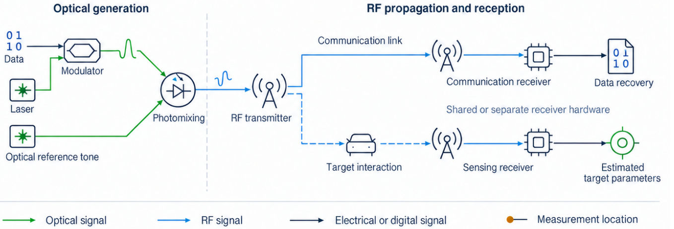
Fig. 3. Conceptual signal paths and measurement locations in O-ISAC. Panel (a) shows alternative fiber and free-space optical paths with direct or coherent reception. Sensing observations may use forward light, backscatter, reflections, or spatial intensity. Panel (b) separates optical generation from radio-frequency (RF) propagation and distinguishes communication and target-interaction paths. Receiver icons represent functional roles with shared or separate hardware. Markers identify launch and received optical power, optical signal-to-noise ratio (OSNR) before photodetection where applicable, electrical signal-to-noise ratio (SNR) after receiver processing, and bit error rate (BER) at data recovery.
