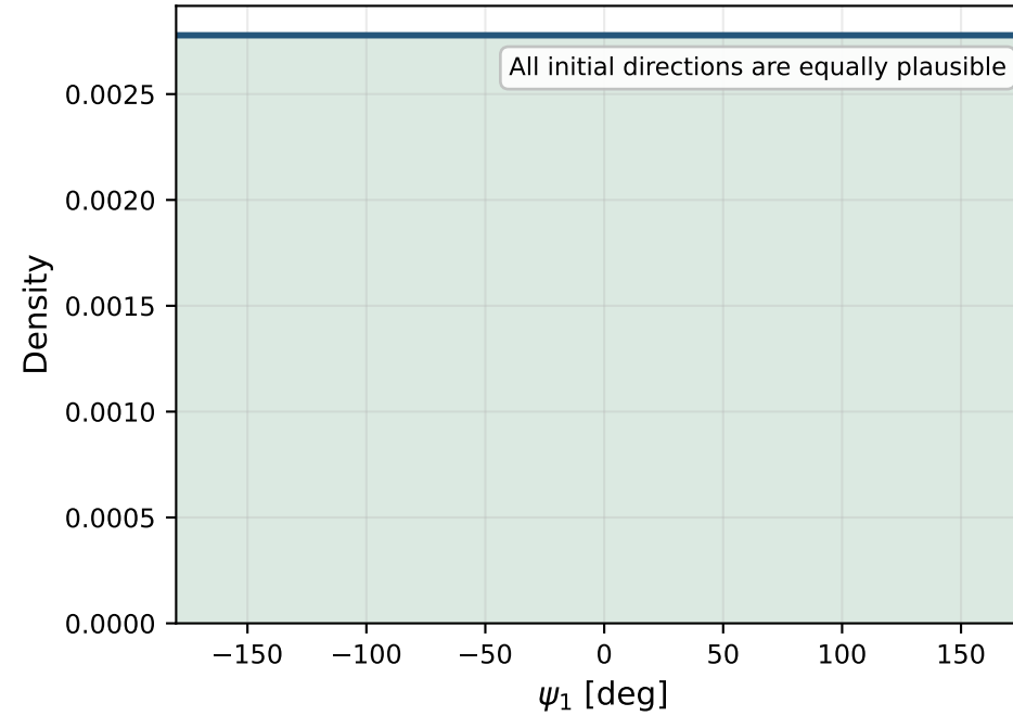
Prior for initial heading
