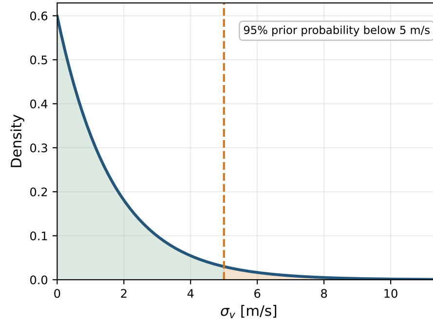
Prior for speed process noise
