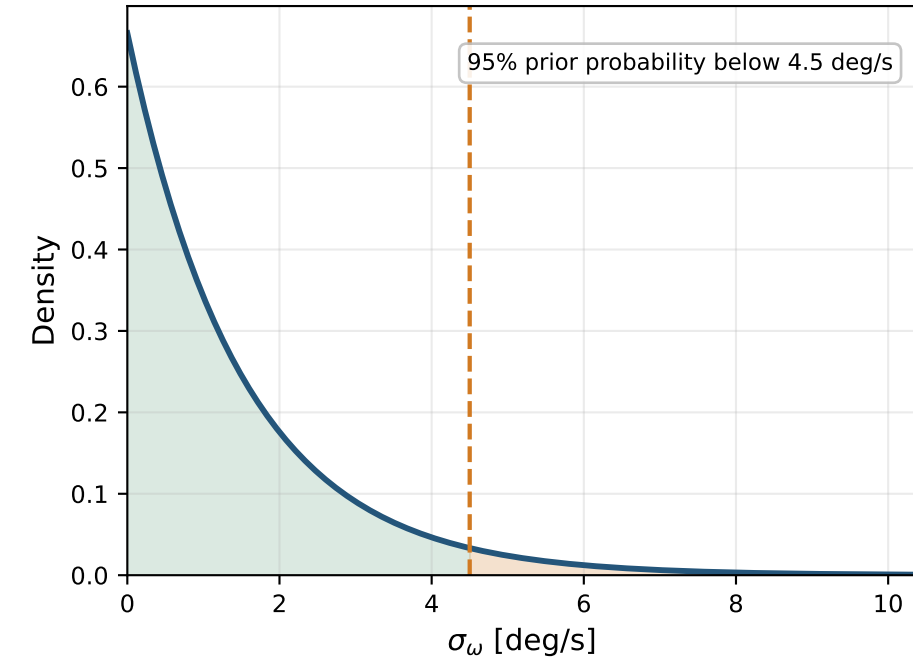
Prior for turn-rate process noise
