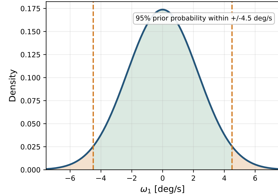
Prior for initial turn rate
