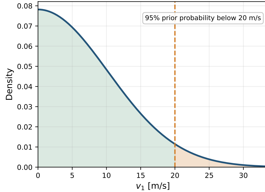
Prior for initial speed
