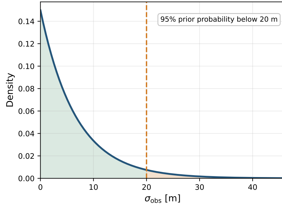
Prior for position observation noise
