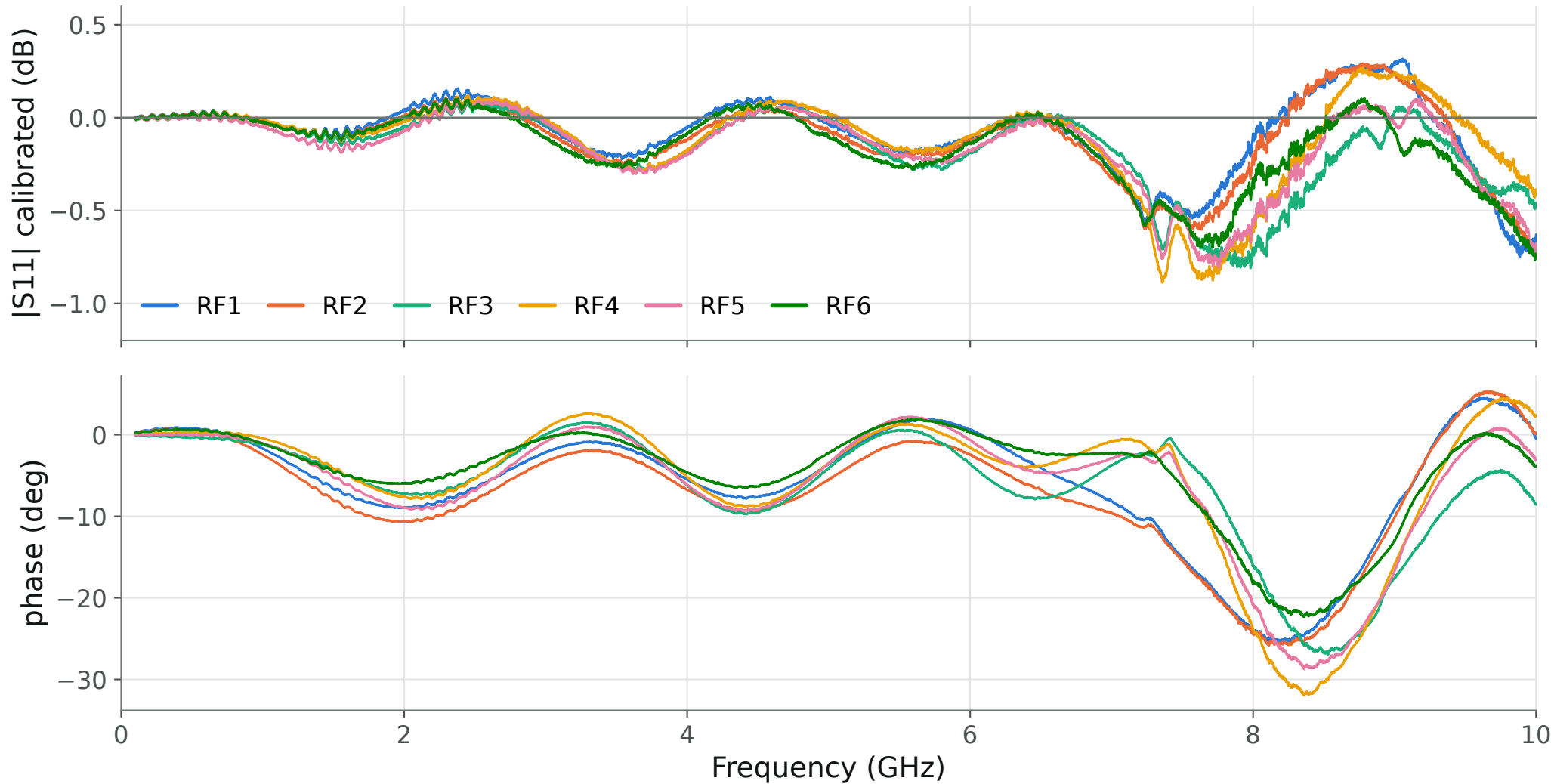
Bench e-cal with NIST's SN0031 295 K definitions: open SMA connector on every port
