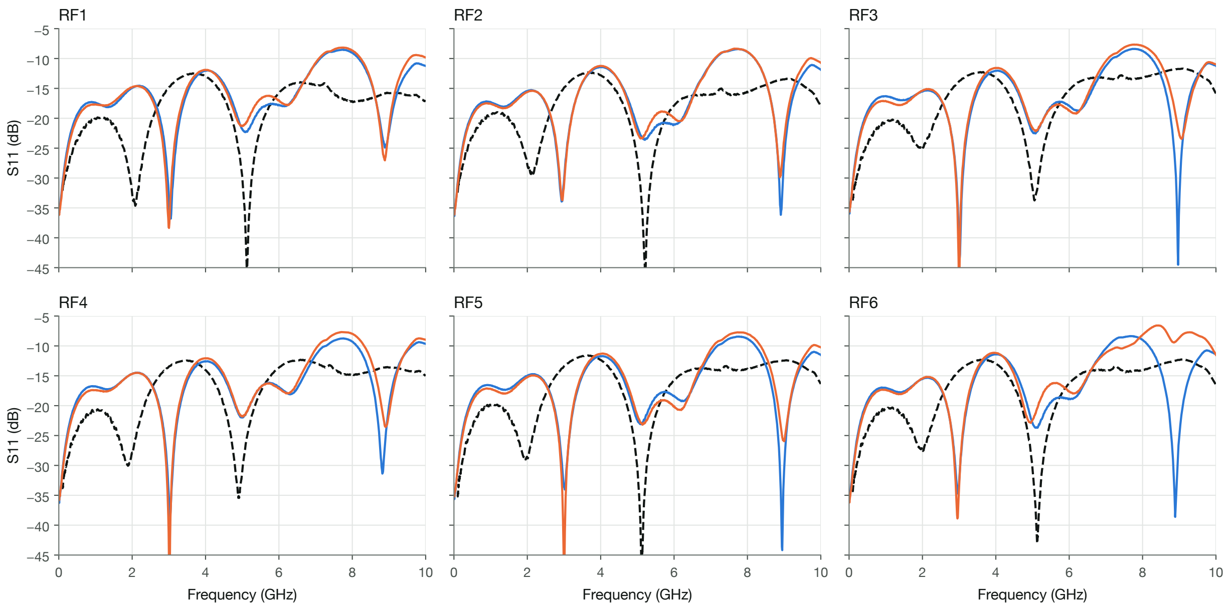
S11: measured switches vs calibrated NIST reference (295 K) — SN77 (measured) — SN78 (measured) - - - NIST SN0031 (calibrated) NIST curve is SN0031's throw path only; measured curves also include the RFC connector section
