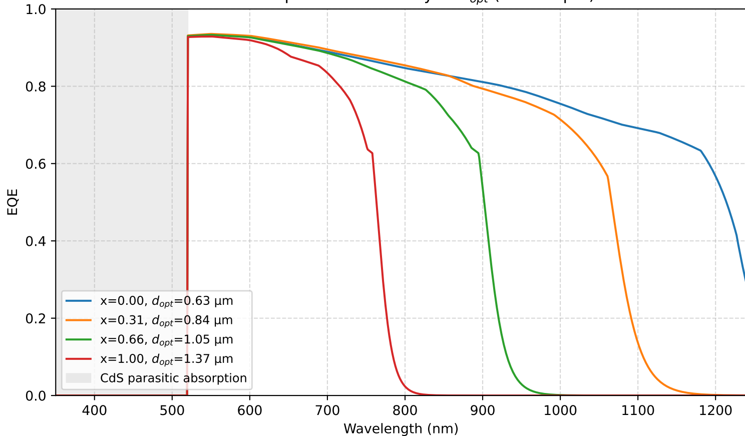
External quantum efficiency at d_{opt} ( L = 1.5 \text{ } \mu\text{m} )
