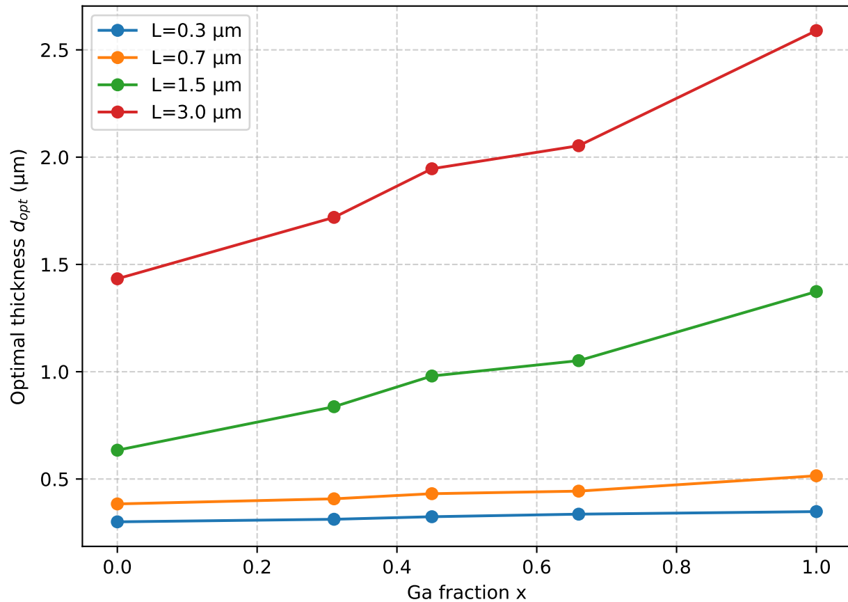
Optimal thickness vs. composition
