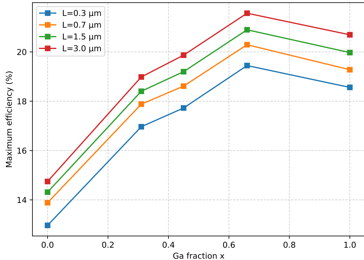
Maximum efficiency vs. composition
